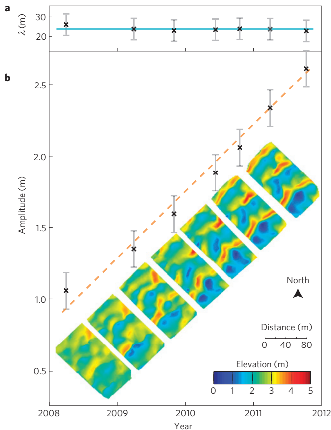
Figure 2 | Development of surface undulations in the open corridor. a , Characteristic wavelength of surface undulations with respect to time. The horizontal line corresponds to a constant wavelength of 23 m. b , Amplitude of surface undulations with respect to time. The dashed line has a slope of 0.41 \text{ m yr}^{-1} . Insets show the evolution of topography. Amplitude and wavelength are calculated from the autocorrelation function of the bed profile using 70 transects. The amplitude is twice the square root of two times the standard deviation. The wavelength is the mean position of the first peak. Error bars are the corresponding standard deviations.
