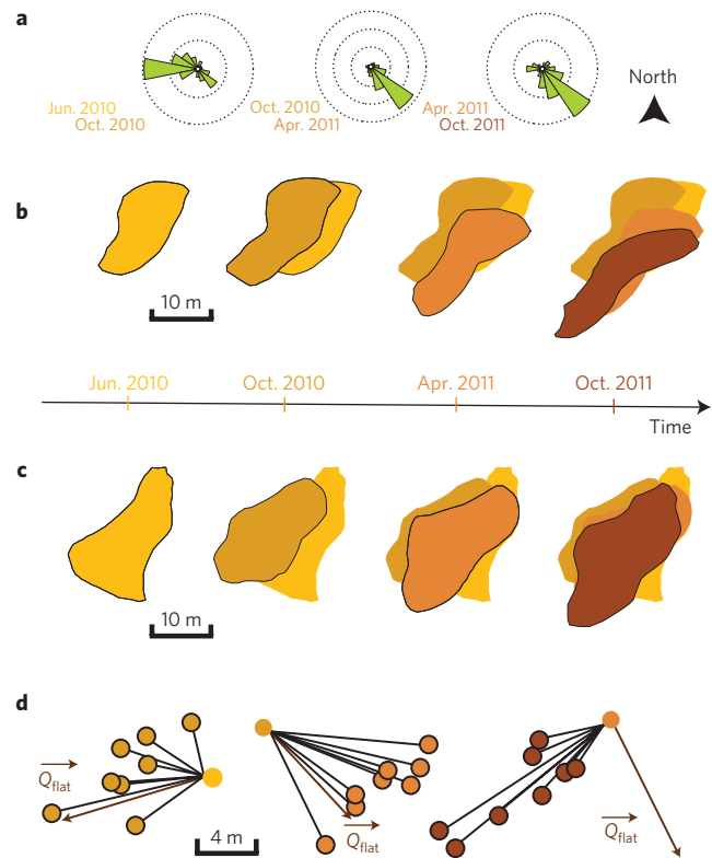
Figure 3 | Morphology and dynamics of individual dunes according to seasonal winds. a , Sand flux roses using the local wind data (Supplementary Information). The three consecutive time periods are characterized by easterly (summer 2010), northwesterly (winter 2010–2011) and bimodal (summer 2011) wind regimes. b,c , Evolution of a dune shape in the open corridor and the closed area. At all times, contours are isolines of equal elevation. d , Horizontal displacements of the centre of mass of eight individual dunes. Brown arrows show the resultant sand flux direction. Note the different phases of dune migration with respect to the wind regime.
