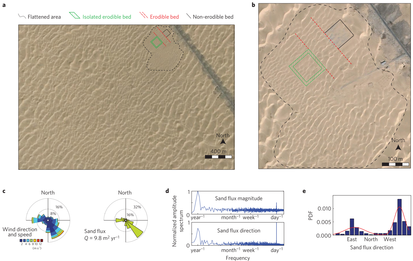
Figure 1 | The landscape-scale experiment site in the Tengger Desert. a, b , The flattened area at two different length scales ( 37^{\circ} 33' 43.5'' N, 105^{\circ} 2' 5.20'' E). The three experimental plots are an open corridor (red), a closed area isolated from external sand flux by a straw chequerboard (green) and a non-erodible bed covered with gravel (black). c , Wind and sand flux roses calculated using the wind data of the local meteorological tower from 1 January 2008 to 31 December 2011 (Supplementary Information). d , Normalized amplitude spectra of the magnitude and the orientation of sand flux. e , The probability density function (PDF) of sand flux orientation and the best fit using a two-component Gaussian mixture model (Methods).
