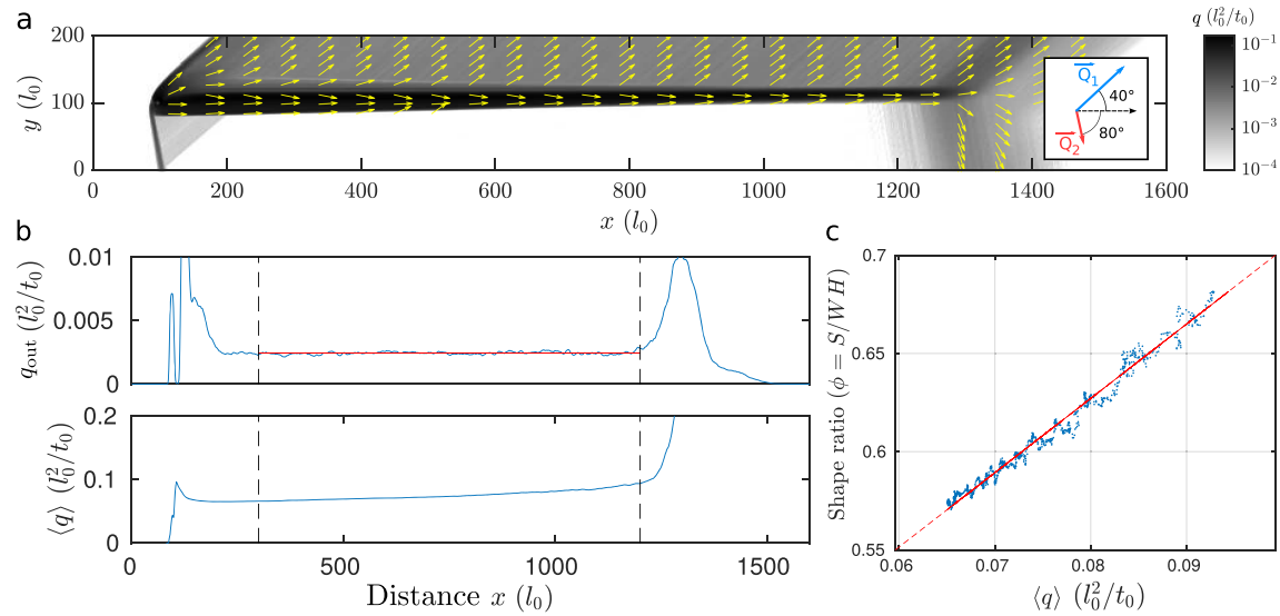
Figure 2. Sand fluxes along a steady linear dune. (a) Intensity (gray scale) and direction (yellow arrows) of the sand flux averaged over 10 wind cycles. (b) Sediment loss q_{out} (top) and mean longitudinal sand flux \langle q \rangle (bottom) along the dune. (c) Dune shape ratio \phi with respect to the mean longitudinal sand flux \langle q \rangle . The solid line shows the best linear fit.
