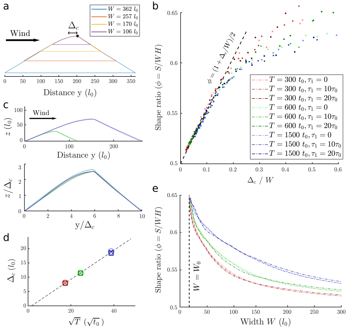
Figure 3. Shape of transverse sections along a steady linear dune. (a) Transverse sections of different width shaped by the same wind regime of period 3,000 t_0 . Cross sections superimpose when matching the crest positions (black point). (b) Shape ratio \phi with respect to the ratio \Delta_c/W for various \{T, \tau_1\} . (c) Transverse sections of different width having same ratio W/\Delta_c = 10 (top). The elevation profiles overlap almost perfectly once normalized (bottom). (d) Crest reversal distance \Delta_c as a function of the square root of the wind period \sqrt{T} . Different symbols are for different values of \tau_1 . (e) Shape ratio \phi with respect to the width W . From (b) to (e), the same color code is used (inset in b), except in (c) where blue elevation profiles are for T = 3,000 t_0 .
