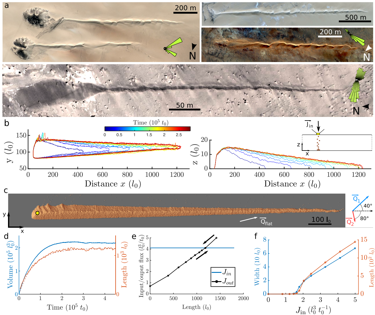
Figure 1. Formation, stabilization, and shape of an elongating linear dune. (a) Elongating linear dunes and sand flux roses in terrestrial dune systems: (top) Niger ( 16^{\circ}52'N , 13^{\circ}20'E , and 18^{\circ}21'N , 13^{\circ}07'E ), (middle) Mauritania ( 23^{\circ}12'N , 10^{\circ}50'W ), (bottom) China ( 39^{\circ}54'N , 94^{\circ}09'E ). Imagery from Google Earth and Maxar. (b) Vertical and horizontal contours of a simulated linear dune elongating from a fixed sand source with a constant influx (see inset). (c) Steady-state dune shape. Transport vectors \vec{Q}_1 and \vec{Q}_2 of primary and secondary winds and resultant \vec{Q}_{flat} = \vec{Q}_1 + \vec{Q}_2 are shown in blue, red, and white, respectively. The black arrow is the predicted dune orientation. The sand source is depicted by the yellow disk. (d) Volume and length of a linear dune as a function of time. The red dashed line shows the prediction. (e) Stability diagram. The steady length is selected when the input ( J_{in} ) and output ( J_{out} ) fluxes balance. (f) Length and maximum width of a steady linear dune with respect to sediment influx.
