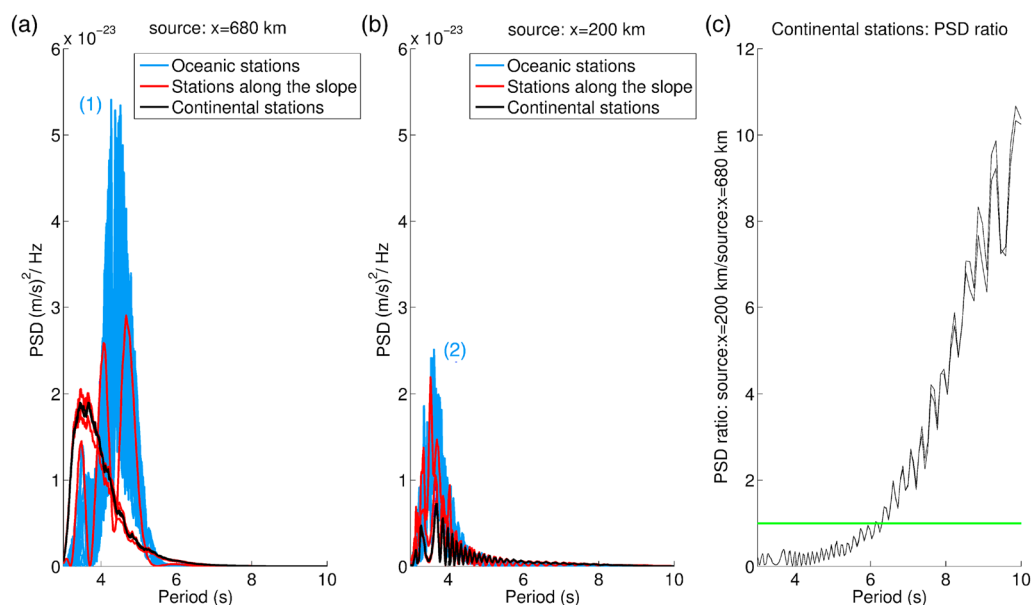
Figure 6. PSD (\text{m/s})^2/\text{Hz} of synthetic seismograms shown in Figure 5 for a source located above (a) shallow water, at x = 680 km, and (b) deep water, at x = 200 km. (c) The ratio between the land-recorded PSD due to a source in deep and shallow water. The same color notation as in Figure 5 has been adopted: blue, red, and black spectra correspond to traces recorded below the seafloor, along the ocean-continent boundary and on land, respectively. Both oceanic (blue) and continental (black) PSDs due to a source in shallow water (Figure 6a) are more amplified than the PSDs due to a source in deep water (Figure 6b). Spectra recorded along the slope (red) show a comparable amplitude. The maximum peak of oceanic PSDs due to a shallow (Figure 6a) and a deep (Figure 6b) water source occurs at different periods, and it is due to different seismic phases. The PSD peak (1) is due to the Airy phase of the fundamental mode in shallow water, whereas the PSD peak (2) is due to the Airy phase of the first overtone in deep water (see Appendix A for more details). (c) The land-recorded PSD due to a source in shallow water is smaller (larger) at periods T > 6 s ( T < 6 s) than the land-recorded PSD due to a source in deep water. The green line in Figure 6c refers to a ratio equal to 1.
