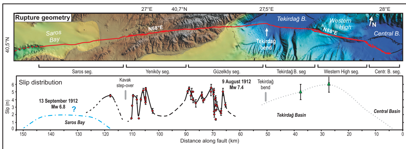
Figure 4. Ganos fault segment (seg.) and A.D. 1912 coseismic slip distribution. Subsegments along fault zone indicate geometrical complexities. The 150-km-long fault (red lines in upper panel) includes 9 August and 13 September earthquake ruptures. Marmara Sea slip values (two triangles in lower panel; Armijo et al., 2005) and inferred dashed line may include penultimate earthquake. Blue dashed line is estimated slip distribution ( \bar{U} = 1.2 m) for Mw 6.8 strike-slip earthquake. B.—Basin (Central).
