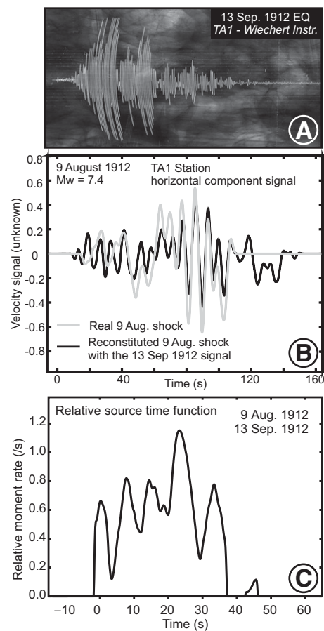
Figure 3. A: Historical seismic record collected and digitized for this study. B: Digitized seismogram of Taranto station (Italy) and waveform modeling showing comparison between real (gray) and reconstituted (black) 9 August 1912 shock. C: Relative source time function of 9 August 1912 and 13 September 1912 earthquakes gives ratio of 0.9–1 in moment magnitude and ~40 s rupture duration.
