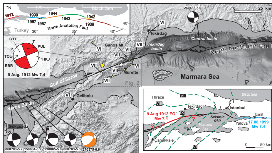
Figure 1. Seismotectonics of western Marmara region. Focal mechanisms are from Harvard Centroid Moment Tensor catalog ( http://www.globalcmt.org/ ; date as day-month-year [e.g., 060703] and M_w indicated at bottom), and A.D. 1912 solution is obtained from P-wave first motions at stations PUL, GTT, EBR, TOL, and HKJ. Offshore fault trace (black lines) is modified from Armijo et al. (2005) and Ustaömer et al. (2008). White and yellow stars are 9 August and 13 September 1912 epicenters, respectively ( \pm 0.1^\circ ; Ambraseys and Jackson, 2000). Roman numerals indicate MSK (maximum intensity in Medvedev-Sponheuer-Karnik scale) intensities of 13 September event (Hecker, 1920). Upper left inset indicates 1912 earthquake location relative to 1939–1999 earthquake sequence. Lower right inset shows isoseismals (dashed lines) of 9 August earthquake (EQ) and Marmara seismic gap (Ambraseys and Finkel, 1987).
