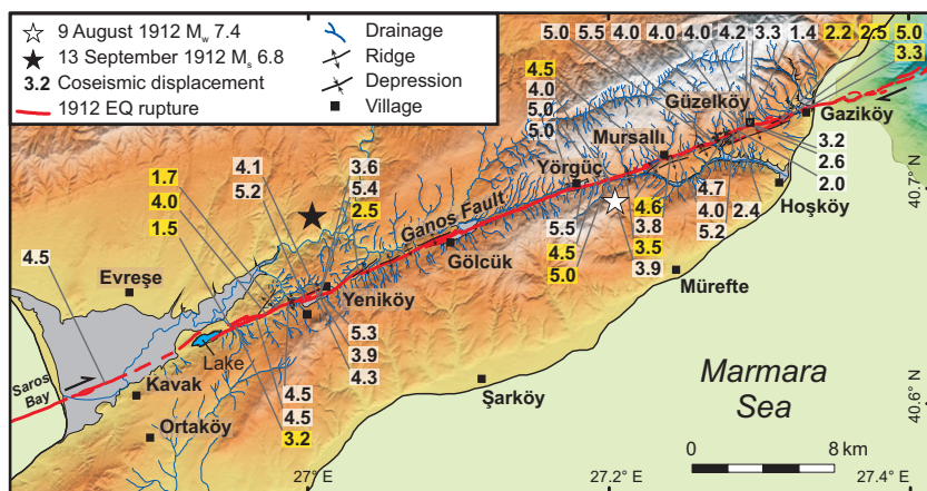
Figure 2. Ganos fault onshore and A.D. 1912 coseismic slip distribution (in meters). Yellow boxes correspond to measures of this study. EQ—earthquake.
