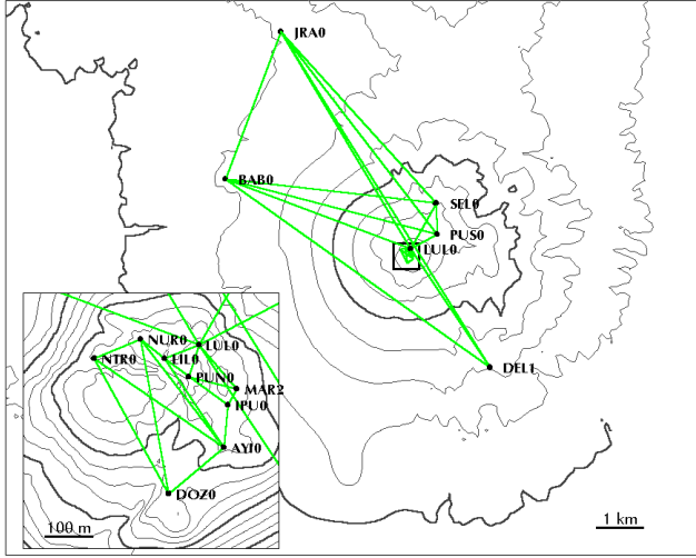
Figure 5. Merapi GPS network and example of baselines pattern measured in March 1997.
