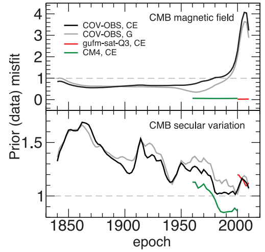
Figure 2. Normalized misfits to the data (prior misfits) \Delta_B (top) and \Delta_S (bottom, see text for definitions), obtained by inverting models COV-OBS, gufm-sat-Q3 and CM4 with priors CE and G. A misfit of 1 (dashed grey line) denotes an acceptable fit (0 is optimal).
