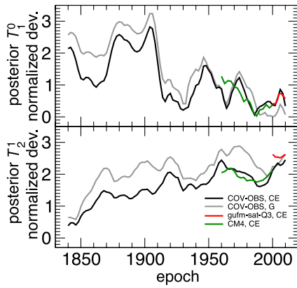
Figure 10. Absolute values of the inverted single-harmonic core surface flow toroidal coefficients T_1^0(r_{\text{CMB}}) and T_2^1(r_{\text{CMB}}) , normalized by their corresponding standard deviations in the numerical dynamo prior.
