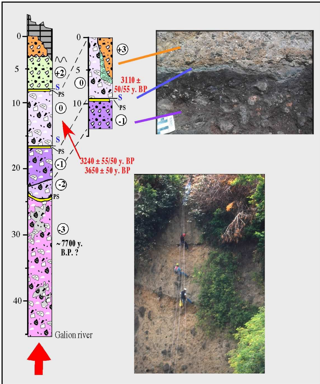
Figure 3. The Fort Delgrès section : A thick sequence of 7 debris avalanche deposits resulting from successive flank-collapse event are observed in the Galion valley. They are separated by more or less developed paleosols and in some cases by lateral directed blast deposits located at the bottom of the associated debris avalanche deposit.
