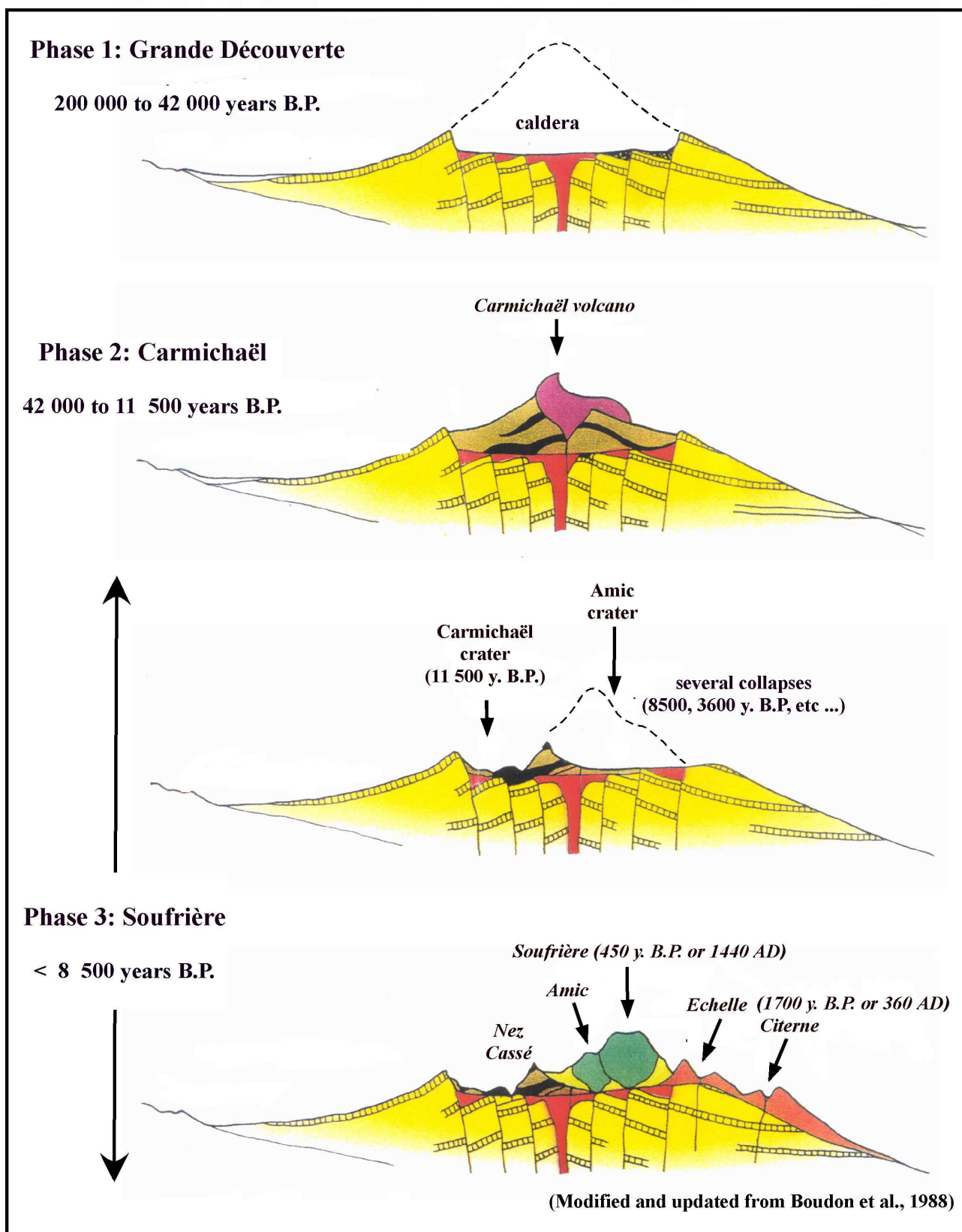
Figure 2. Simplified geological cross-sections showing the evolution of the Grande Découverte – Soufrière volcanic complex (modified after Boudon et al., 1988)
