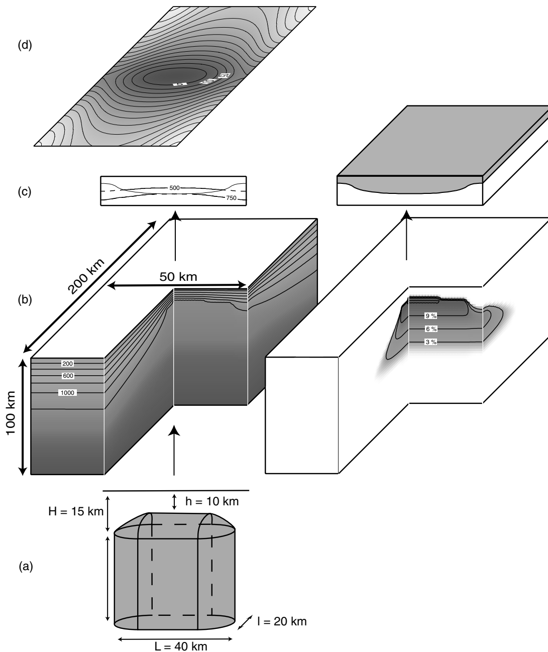
Figure 4. Model outputs. (a) The ‘best-fitting’ intrusion geometry. (b) Modelled thermal structure (left) and distribution of the partial melting rate (right). (c) Along-axis crustal sections. Left : the thin line represents the Moho, the thick lines 500 and 750 °C isotherms, marking the maximal depth of the earthquake in the crust and in the mantle, respectively. At the segment centre the 500 °C isotherm is 4 km below the seafloor. At the segment ends, the 750 °C isotherm is 8 km deep. Right : crustal thickness. The crust is 6 km thick at the the segment centre and 2–3 km thick at the ends. (d) Modelled MBA reproducing the circular shape (‘bull’s eye’) observed over the segment centre. From the centre towards the segment ends, the \Delta MBA amplitude is 23 mGal.
