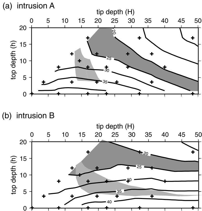
Figure 3. Determination of the ‘best-fitting’ parameters h and H , in the cases of intrusion shape A and B (see caption of Fig. 2 for their definition) Crosses show the couples ( h , H ) for which the geophysical outputs are calculated. The values of these outputs are interpolated within the range of investigated h and H . Thick lines represent the \Delta MBA between segment centres and segment ends. The lighter grey region represents the range of parameters h and H accounting for the observed maximal depths of the earthquakes. The darker grey region represents the range of parameters h and H accounting for the observed \Delta MBA amplitude.
