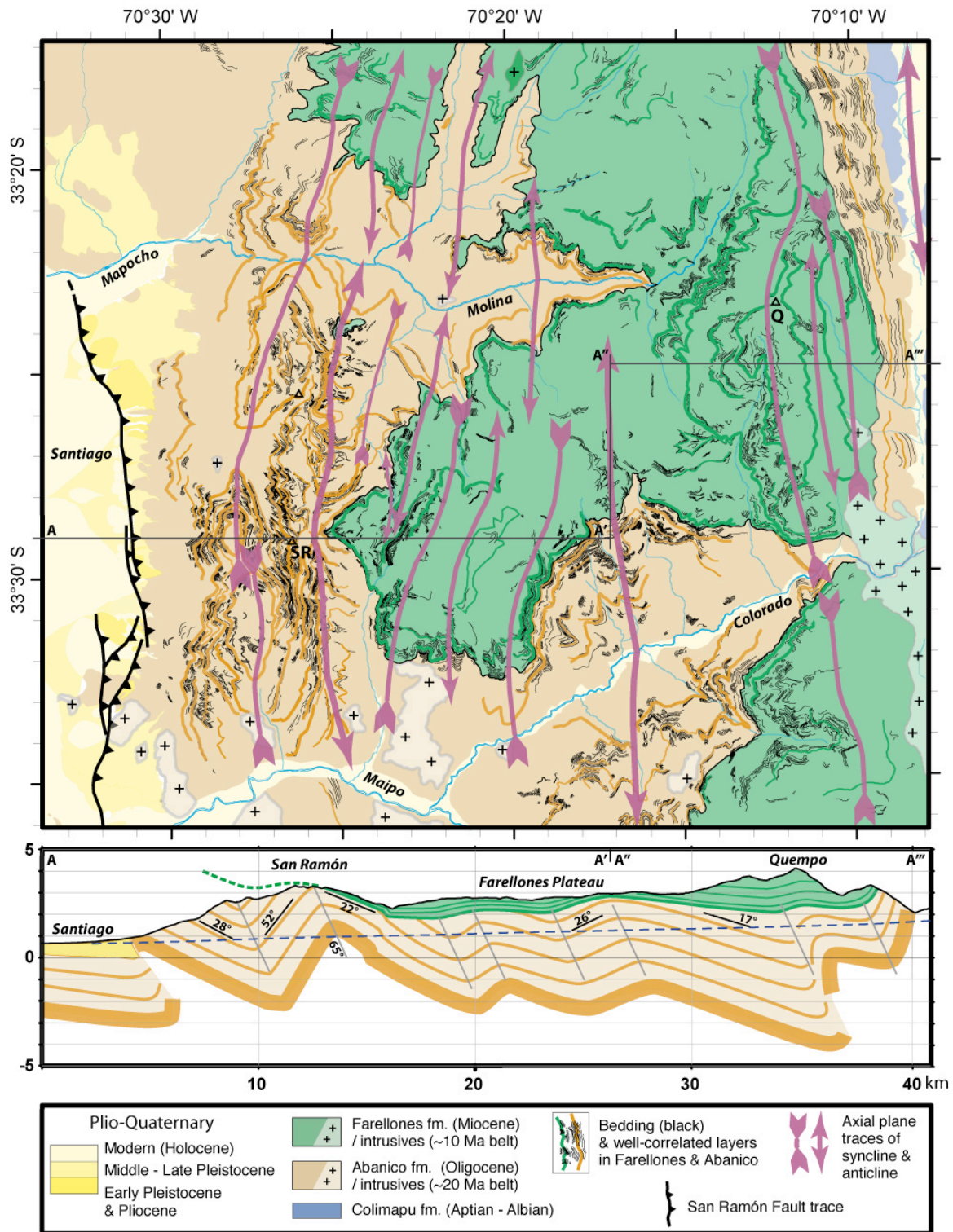
Fig. 3b. Morphology and structure of the West Andean Front and the western Principal Cordillera facing Santiago. Structural Map of the San Ramón - Farellones Plateau region and corresponding E-W section (see location in Fig. 2b). Bedding attitudes are determined by mapping systematically over a DEM the most visible layers (thin black lines) with overall horizontal resolution of 30 m, using SPOT satellite imagery, aerial photographs and field observations. Well-correlated layers (correlated over distances of kilometres) are indicated by thicker brown and green lines (in Abanico and Farellones Formations, respectively). The basal contact of Farellones fm. has been modified from Thiele [1980], to be consistent with details of the mapped layered structure. The trace of axial planes of main folds is indicated. SR locates summit of Cerro San Ramón (3249 m); Q, summit of Cordón del Quempo (4156 m). Section shift (from AA' to A''A''') is chosen to better represent the fold structure of San Ramón and Quempo. Bedding and axial plane attitudes in the section are obtained by projection of structural elements mapped over the DEM, so directly constrained by the surface geology between the high mountainous topography and the longitudinal profile of Colorado river (dashed blue), and extrapolated below that level. The geometry of base of Abanico fm. is consistent with the structure observed in the upper part of the section, and it has been tentatively interpolated between where it pinches out with shallow eastward dip beneath sediment of the Santiago Basin, and its outcrop with steep westward dip in the Olivares river valley, east of Quempo.
