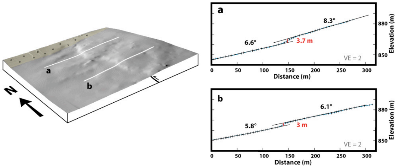
Fig. 7. Morphology of most recent scarp across young (Holocene?) alluvial fan. a. DEM with 2 m horizontal resolution; 0.1 m vertical precision, based on a differential DGPS survey covering an area about 400 x 300 m 2 (location shown in Figs. 4 and 7). The younger alluvium to the North (yellow) conceals the scarp. b. Profiles show a scarp 3-4 m high that may have resulted from a single event. Vertical exaggeration is 2. Profile symbols as in Fig. 6. The GPS data are not referenced, so the elevation base is within error of about \pm 10 m.
