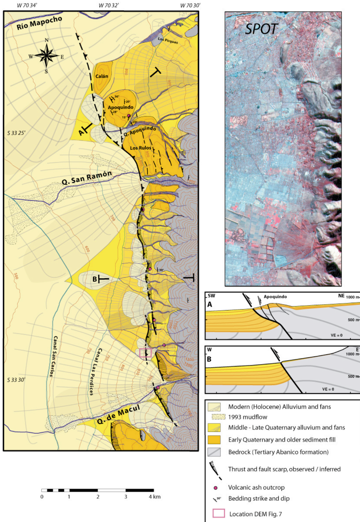
Fig. 4. Map, satellite SPOT image and sections describing the San Ramón Fault and its piedmont scarp in the eastern districts of Santiago. Map and SPOT image cover same area (shown in Figs. 2b and 3a). Sections tentatively interpreted across the fault (labelled A and B) are located in the map. The San Ramón Fault trace is at the foot of a continuous scarp east of which the piedmont is uplifted and incised by streams. The more incised Cerros Calán, Apoquindo and Los Rulos (to the N) expose an anticline made of Early Quaternary sediments, cored by bedrock of the Abanico Formation and possibly cut by subsidiary thrusts, as those better exposed and mapped in Cerro Los Rulos (illustrated in section A). The gently sloping piedmont that is uplifted in the central part of the segment (section B) is covered with Middle-Late Pleistocene alluvium containing lenses of volcanic ash correlated with Pudahuel ignimbrites (see text). The map has been compiled and geo-referenced at 1:25.000 scale, from original mapping on a DEM at 1:5.000 scale (shown in Fig. 6).
