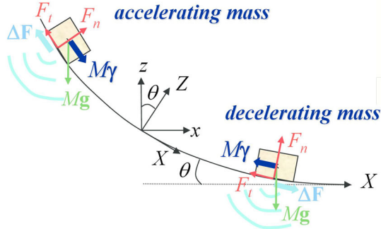
(a) Sliding block model
