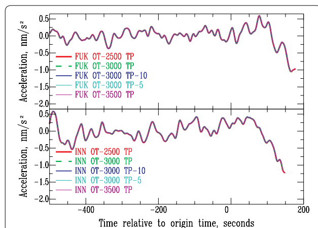
Fig. 2 Robustness of the V17 data processing illustrated for two stations of the F-net network. FUK (top) and INN (bottom) are STS1 and STS2 sensors, respectively. For each sensor, the curves show the obtained vertical acceleration signals for different choices of the original time window. These choices can be read in the name given to each curve: the negative number following “OT” gives the starting time (in s) of the window relative to the Tohoku earthquake origin time; the negative number following “TP” gives the ending time (in s) of the window relative to the P-wave arrival time at each station. No differences can be observed in the resulting accelerations in the 0.002–0.03 Hz frequency band
