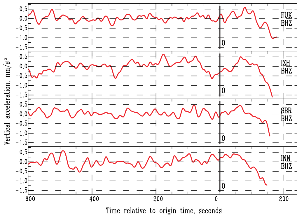
Fig. 3 Objective comparison between PEGS signals observed in Southwest Japan. All signals have been processed using the V17 procedure and the FUK signal (top row) is therefore exactly the same as the one shown in Figs. 1 and 3 of V17. The other three signals are the only other ones among the stations shown in Fig. 2 of K19 that meet the quality criterion of V17. All signals show consistent PEGS, supporting the use of only one of them (FUK) in the V17 study. Due to its correct data processing and appropriate noise considerations, this figure is the logical alternative to Fig. 2b of K19
