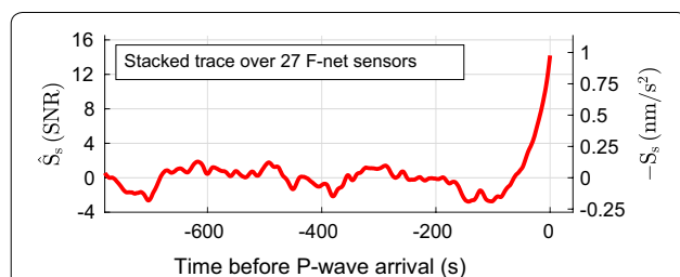
Fig. 4 Consistency between observed PEGS amplitudes and V17 modeling. Stacked trace (station-averaged vertical acceleration) of the same 27 sensors considered in Fig. 7a of K19, but deconvolving the data by the instrument response (as done in V17) before stacking. Note that the stacked trace S_s is shown with an opposite sign (scale to the right). The stack SNR (scale to the left) is defined as the ratio between |S_s| and the standard deviation of noise calculated in the 10 min preceding earthquake origin time. At the P wave arrival, S_s \sim -1 \text{ nm/s}^2 and \text{SNR} \sim 14
