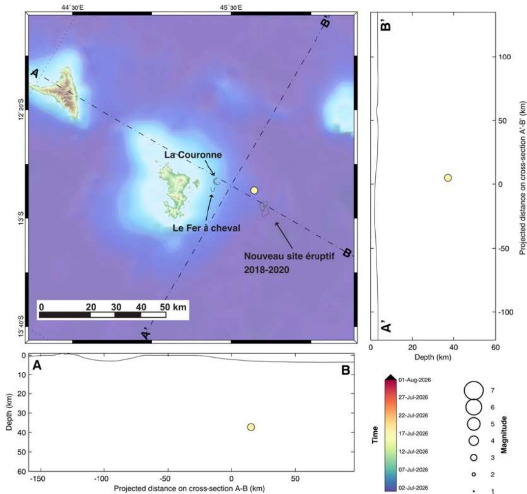
Mayotte time evolution - all area © MAYOBS1 2019/SHOM 2016/SRTM/ETOPO, 2026 +© IPGP/ReVoSiMa, 2026
