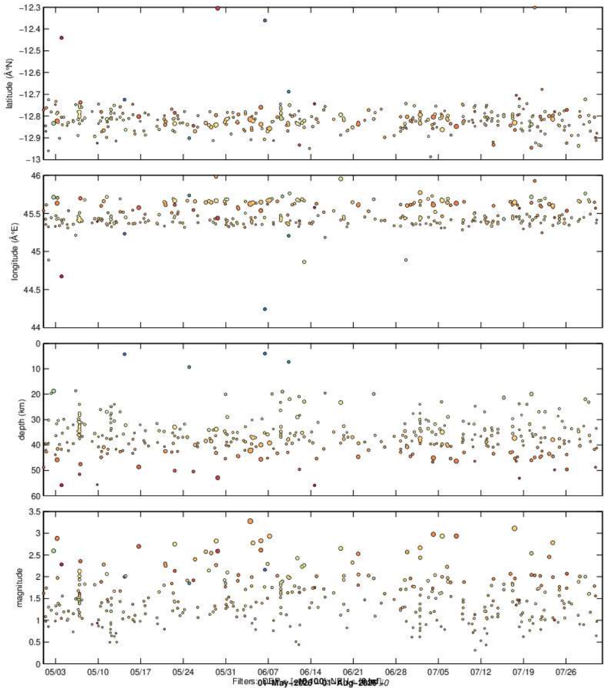
Mayotte time evolution – all area © MAYOBS1 2019/SHOM 2016/SRTM/ETOPO, 2026 +© IPGP/ReVoSiMa, 2026
