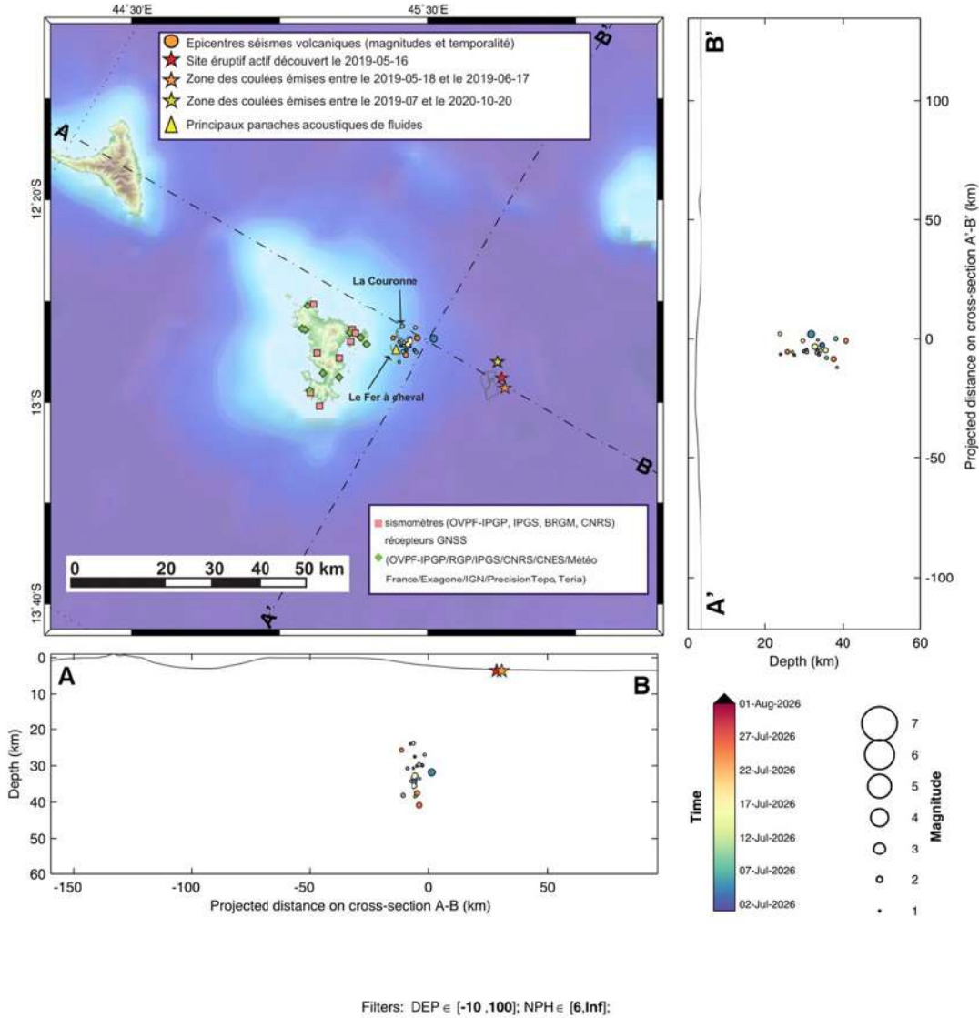
Mayotte time evolution - all area © MAYOBS1 2019/SHOM 2016/SRTM/ETOPO, 2026 +© IPGP/ReVoSiMa, 2026
