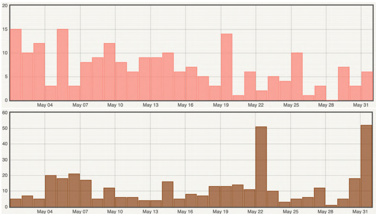
Figure 1: Number of (top) shallow volcano-tectonic earthquakes and (bottom) rockfalls per day recorded in May 2023 (© OVPF-IPGP).
