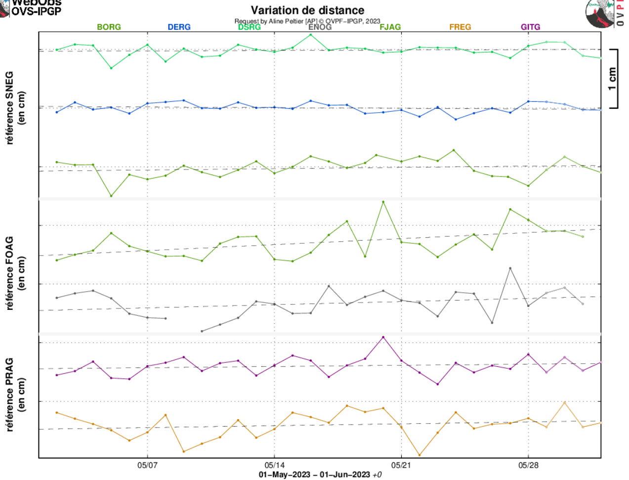
Figure 4: Ground deformation records over the course of May 2023 (in case of eruptive or intrusive periods, red and green bars represent eruptions and intrusions, respectively). The time series plots show the changes in distance between pairs of GPS stations located around the Dolomieu summit crater (reference: SNEG; top graph), the terminal cone (reference: FOAG; middle graph) and the Enclos Fouqué caldera (reference: PRAG; bottom graph), from north to south (see location in Figure 5). Increasing distances (or baseline elongation) indicate volcano inflation, while decreasing distances (or baseline contraction) reflect edifice deflation (© OVPF-IPGP).
