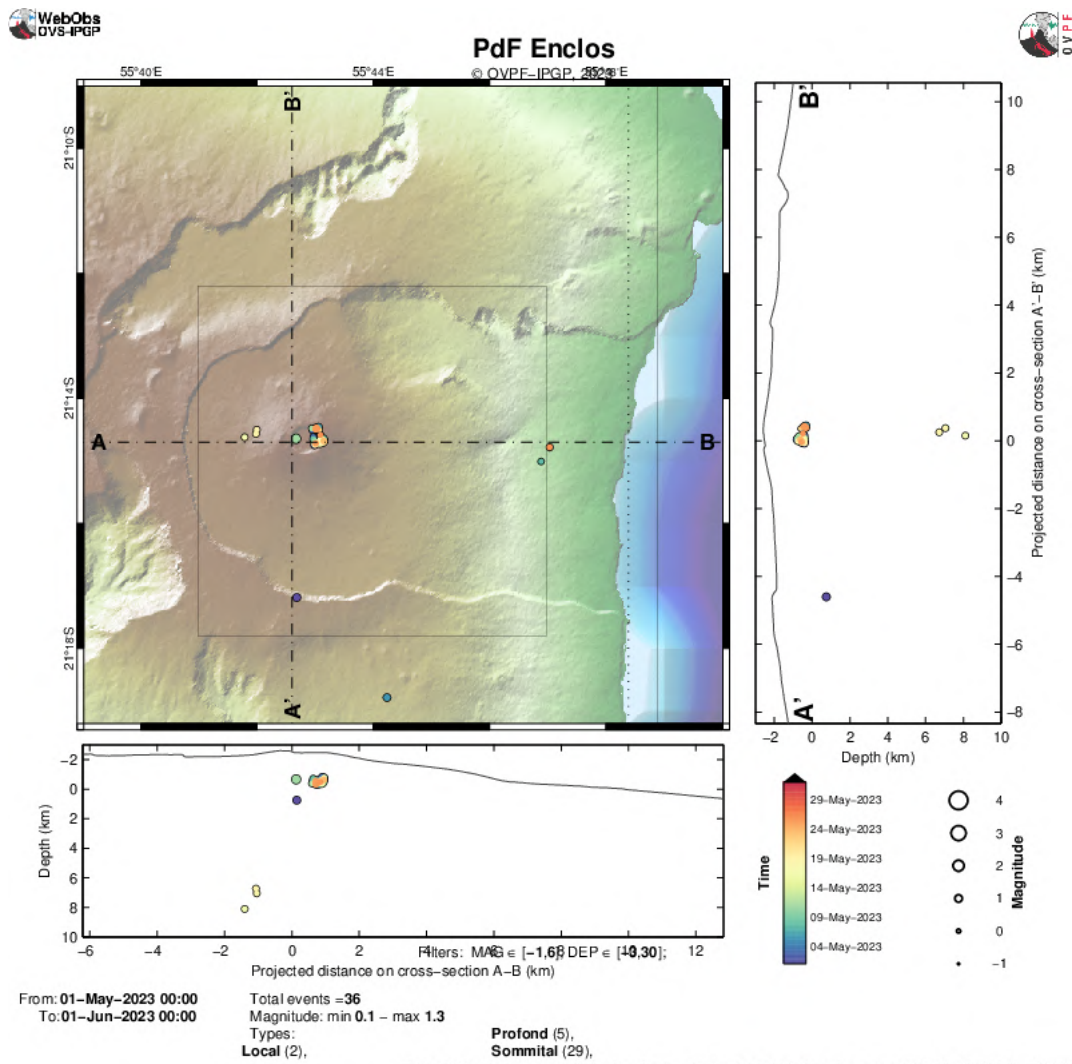
Figure 2: Seismicity below Piton de la Fournaise in May 2023. Location map (epicenters) and north-south and east-west cross-sections (hypocenters) of earthquakes as recorded by OVPF-IPGP. Only manually located earthquakes are shown on the map (© OVPF-IPGP).
