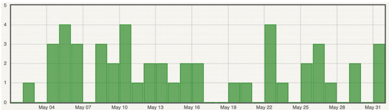
Figure 9: Number of local earthquakes (La Réunion island) per day recorded in May 2023 (© OVPF-IPGP).
