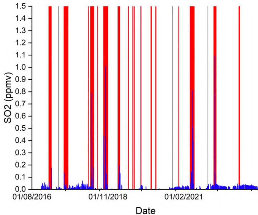
Figure 8: Raw (in blue) concentrations of SO 2 in the atmosphere at the summit of Piton de la Fournaise (MultiGaS station). Red bars: eruptions; Gray bars: intrusions (© OVPF-IPGP).
