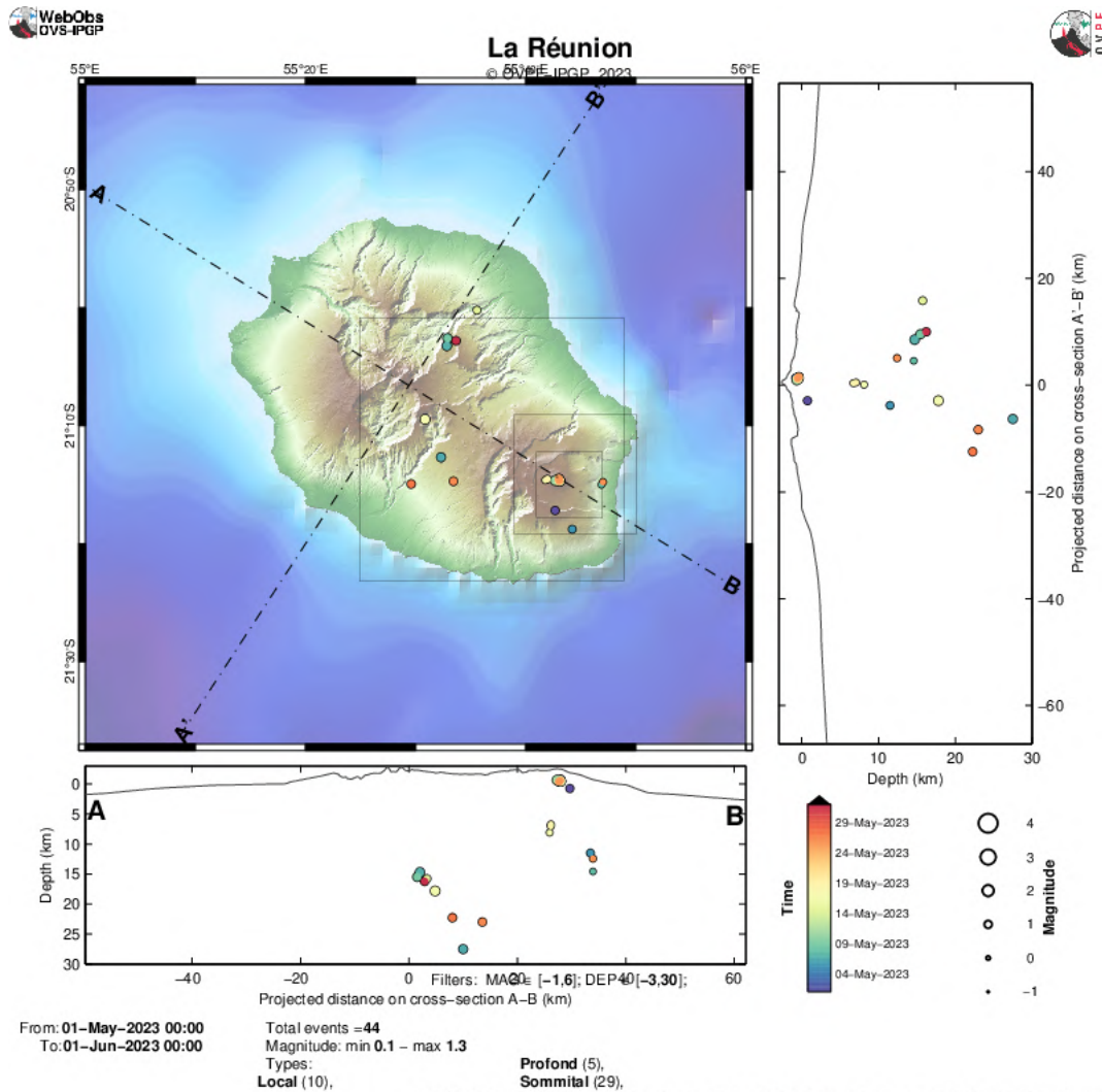
Figure 10: Seismicity below La Réunion in May 2023. Location map (epicenters) and north-west – south-east and south-west – north-east cross-sections (hypocenters) of earthquakes as recorded by OVPF-IPGP. Only localizable earthquakes are shown on the map (© OVPF-IPGP).
