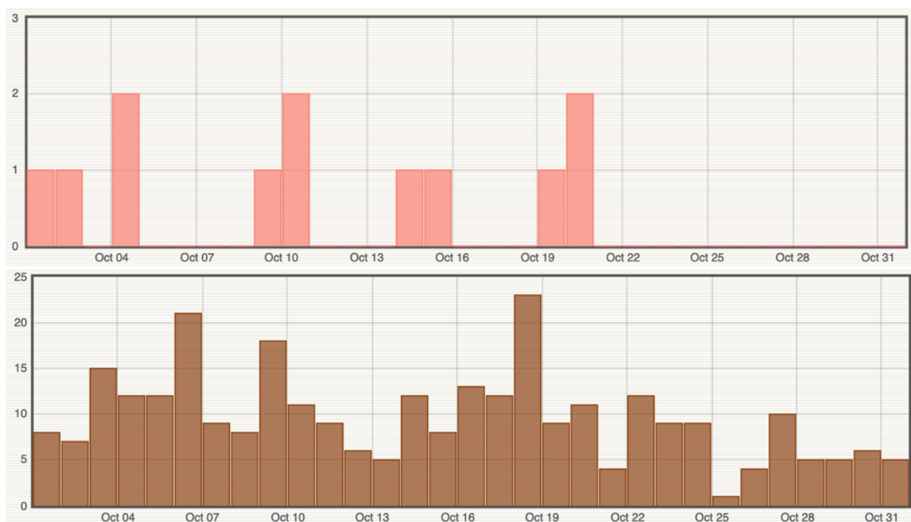
Figure 1: Number of (top) shallow volcano-tectonic earthquakes and (bottom) rockfalls per day recorded in October 2023 (© OVPF-IPGP).
