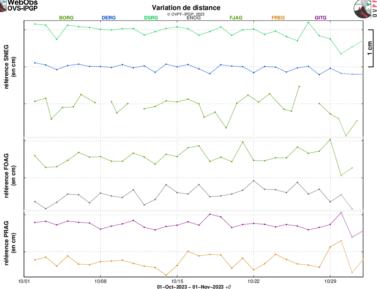
Figure 4: Ground deformation records over the course of October 2023 (in case of eruptive or intrusive periods, red and green bars represent eruptions and intrusions, respectively). The time series plots show the changes in distance between pairs of GPS stations located around the Dolomieu summit crater (reference: SNEG; top graph), the terminal cone (reference: FOAG; middle graph) and the Enclos Fouqué caldera (reference: PRAG; bottom graph), from north to south (see location in Figure 5). Increasing distances (or baseline elongation) indicate volcano inflation, while decreasing distances (or baseline contraction) reflect edifice deflation (© OVPF-IPGP).
