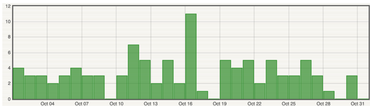
Figure 8: Number of local earthquakes (La Réunion island) per day recorded in October 2023 (© OVPF-IPGP).
