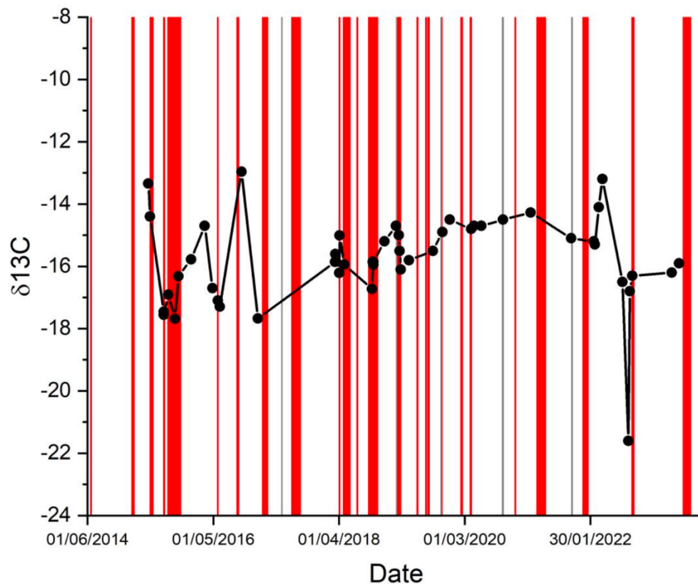
Figure 8: Carbon isotope ( \delta^{13}\text{C} ) variations in \text{CO}_2 from soil gas emitted from the control point with the highest flux in the proximal area (control point: GIT0).
