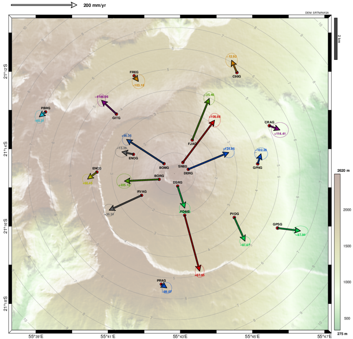
Figure 6: Map of ground displacements (expressed in velocity, mm/yr) recorded between November 1 and 30, 2023 by the OVPF-IPGP permanent GPS network. Horizontal displacements are represented in vector form and vertical displacements are indicated by numerical values in color (© OVPF-IPGP).
