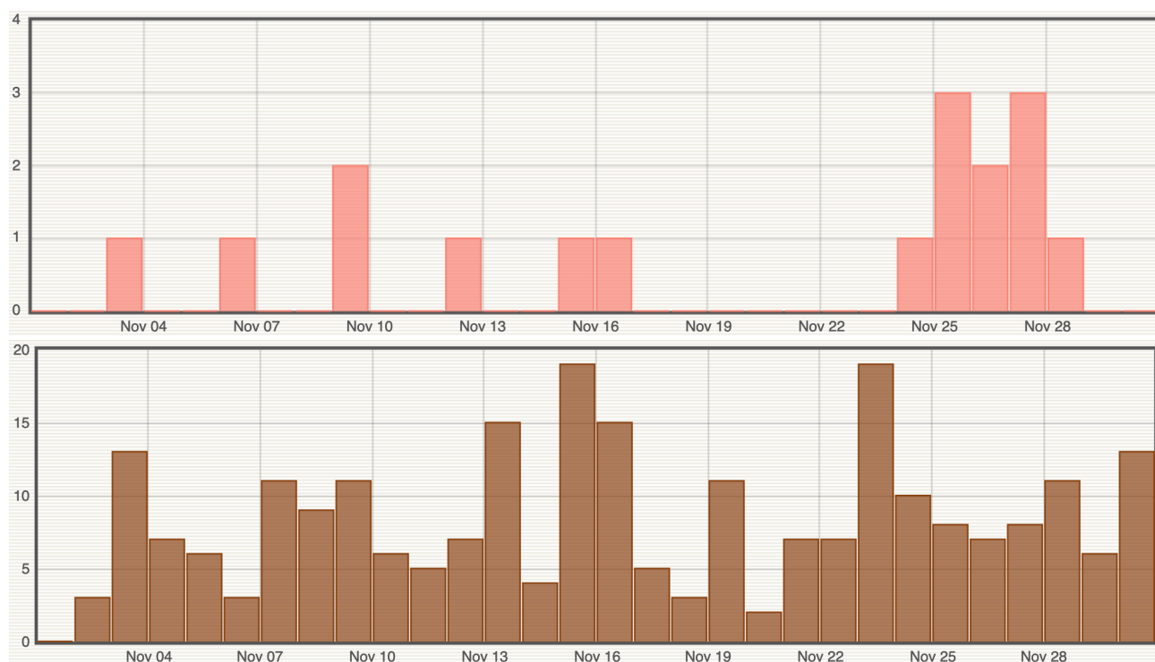
Figure 1: Number of (top) shallow volcano-tectonic earthquakes and (bottom) rockfalls per day recorded in November 2023 (© OVPF-IPGP).
