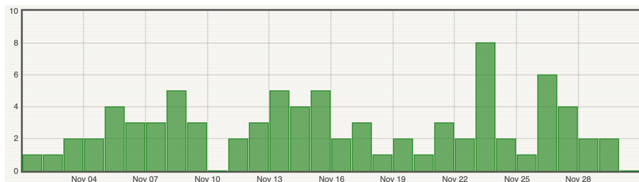
Figure 9: Number of local earthquakes (La Réunion island) per day recorded in November 2023 (© OVPF-IPGP).
