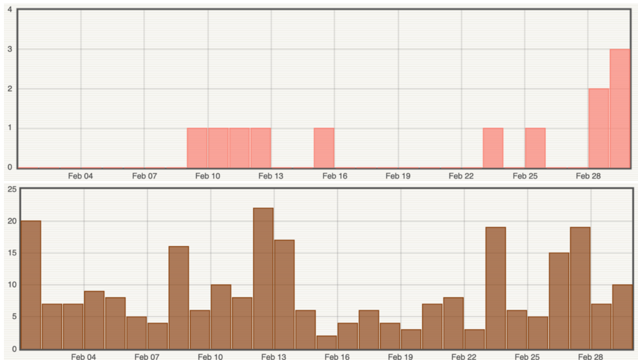
Figure 1: Number of (top) shallow volcano-tectonic earthquakes and (bottom) rockfalls per day recorded in February 2024 (© OVPF-IPGP).
