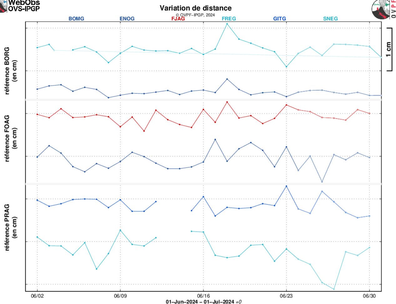
Figure 4: Ground deformation records over the course of June 2024 (in case of eruptive or intrusive periods, red and green bars represent eruptions and intrusions, respectively). The time series plots show the changes in distance between pairs of GPS stations located around the Dolomieu summit crater (reference: BORG; top graph), the terminal cone (reference: FOAG; middle graph) and the Enclos Fouqué caldera (reference: PRAG; bottom graph), from north to south (see location in Figure 5). Increasing distances (or baseline elongation) indicate volcano inflation, while decreasing distances (or baseline contraction) reflect edifice deflation (© OVPF-IPGP).
