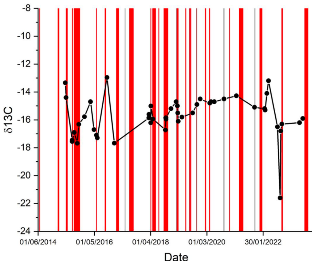
Figure 7: Carbon isotope ( \delta^{13}\text{C} ) variations in CO 2 from soil gas emitted from the control point with the highest flux in the proximal area (control point: GITN).
