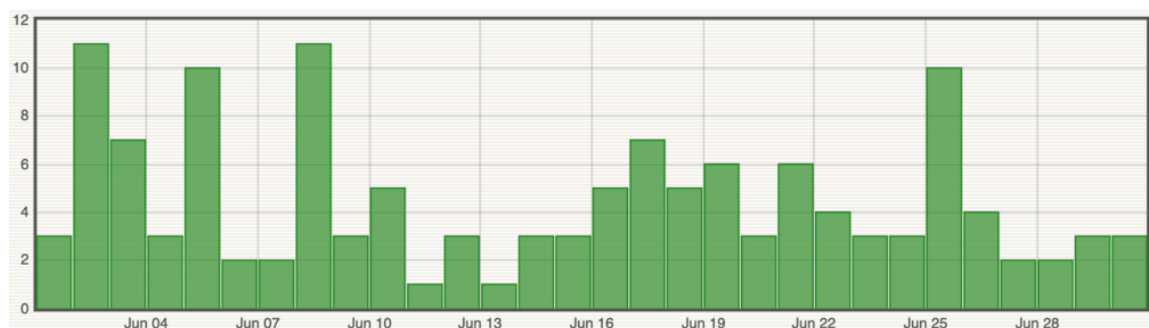
Figure 8: Number of local earthquakes (La Réunion island) per day recorded in June 2024 (© OVPF-IPGP).
