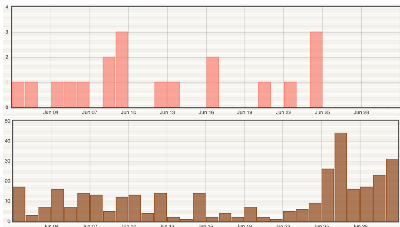
Figure 1: Number of (top) shallow volcano-tectonic earthquakes and (bottom) rockfalls per day recorded in June 2024 (© OVPF-IPGP).
