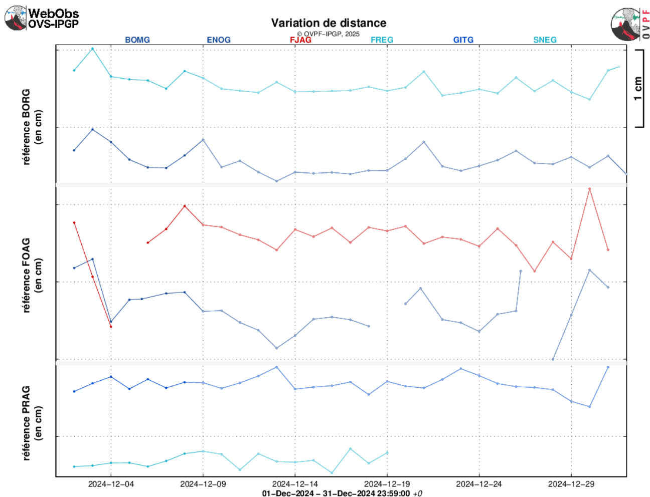
Figure 4: Ground deformation records over the course of December 2024 (in case of eruptive or intrusive periods, red and green bars represent eruptions and intrusions, respectively). The time series plots show the changes in distance between pairs of GPS stations located around the Dolomieu summit crater (reference: BORG; top graph), the terminal cone (reference: FOAG; middle graph) and the Enclos Fouqué caldera (reference: PRAG; bottom graph), from north to south (see location in Figure 5). Increasing distances (or baseline elongation) indicate volcano inflation, while decreasing distances (or baseline contraction) reflect edifice deflation (© OVPF-IPGP).
