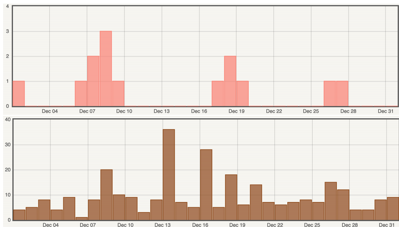
Figure 1: Number of (top) shallow volcano-tectonic earthquakes and (bottom) rockfalls per day recorded in December 2024 (© OVPF-IPGP).
