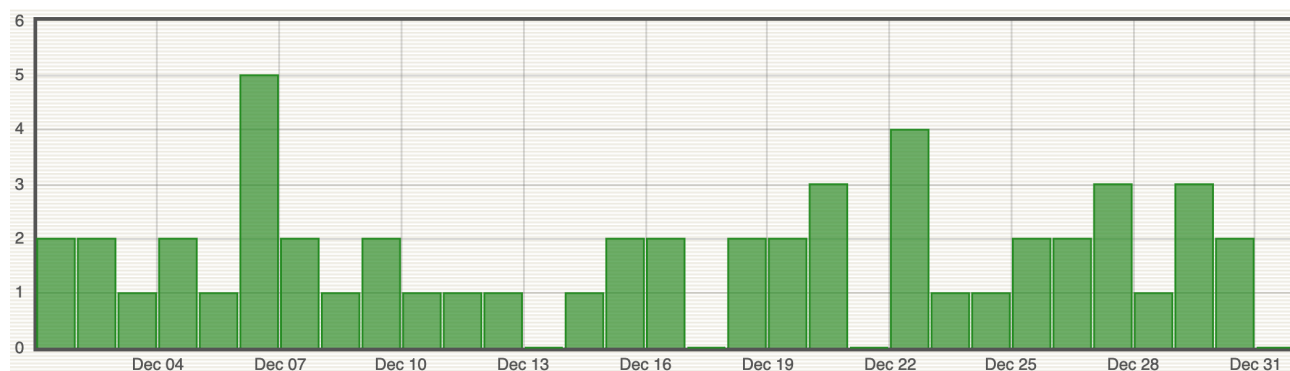
Figure 9: Number of local earthquakes (La Réunion island) per day recorded in December 2024 (© OVPF-IPGP).
