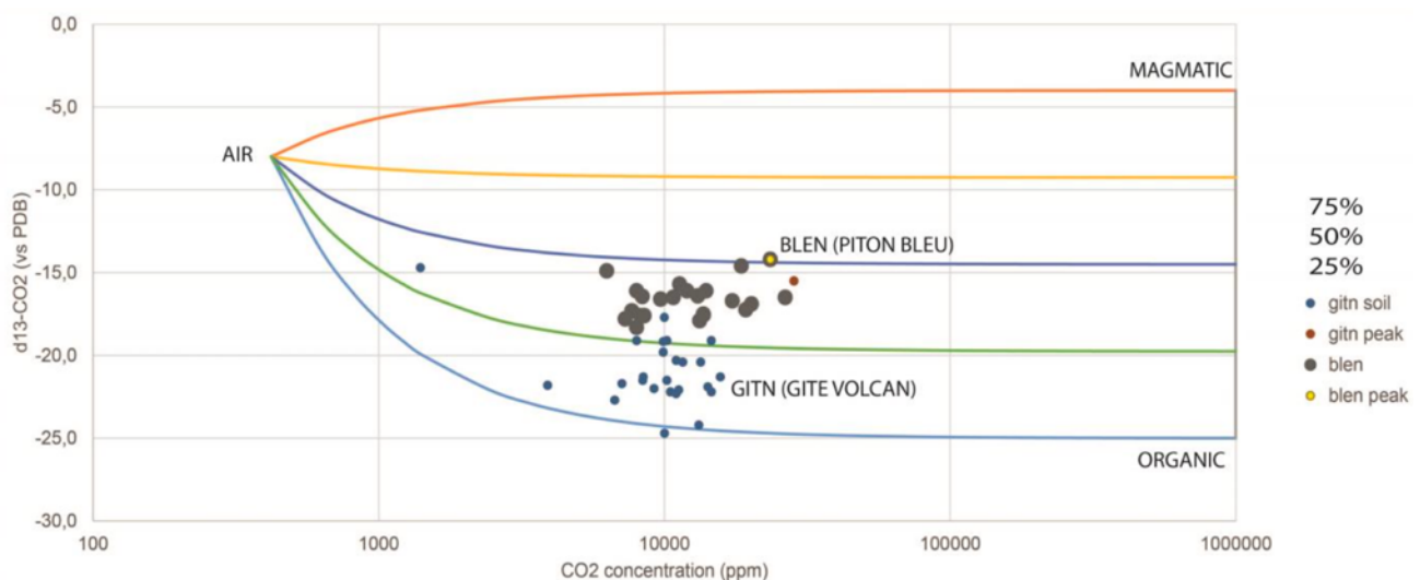
Figure 7: Carbon isotope ( \delta^{13}\text{C} ) variations in CO 2 from soil gas emitted from a proximal (GITN) and distal (BLEN) station. Measurements performed at the beginning (March 2024) of the peak phase in CO 2 emissions do not show a strong increase in the percentage of magmatic contribution.
