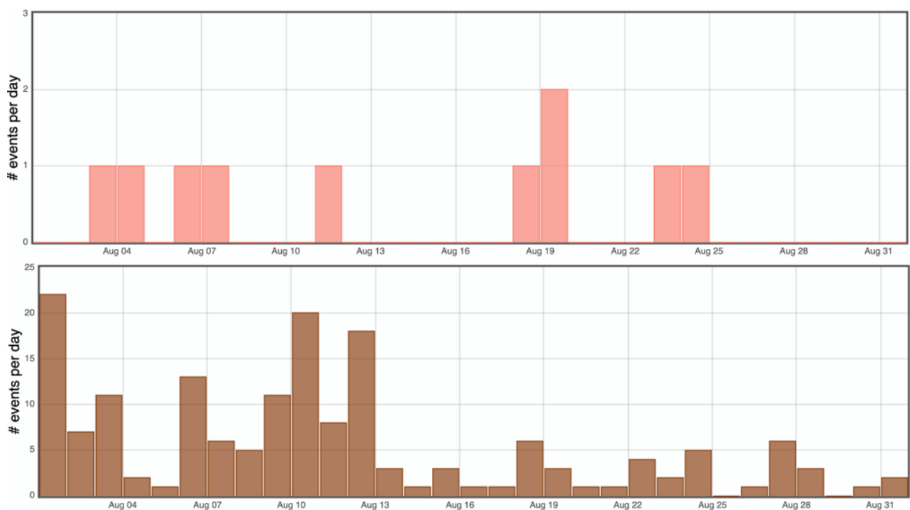
Figure 1: Number of (top) shallow volcano-tectonic earthquakes and (bottom) rockfalls per day recorded in August 2025 (© OVPF-IPGP).
