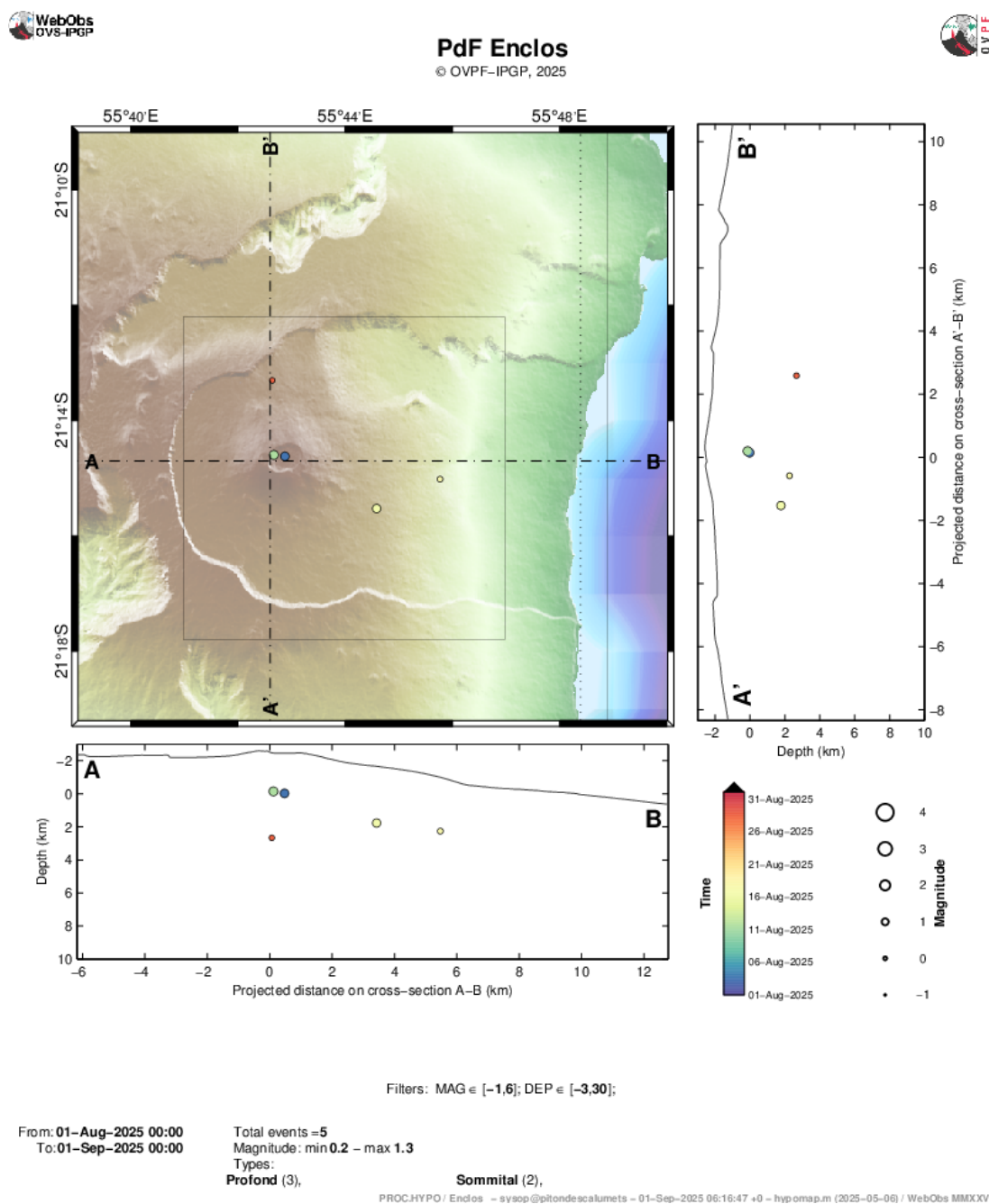
Figure 2: Seismicity below Piton de la Fournaise in August 2025. Location map (epicenters) and north-south and east-west cross-sections (hypocenters) of earthquakes as recorded by OVPF-IPGP. Only manually located earthquakes are shown on the map (© OVPF-IPGP).
