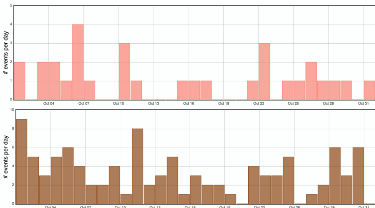
Figure 1: Number of (top) shallow volcano-tectonic earthquakes and (bottom) rockfalls per day recorded in October 2025 (© OVPF-IPGP).
