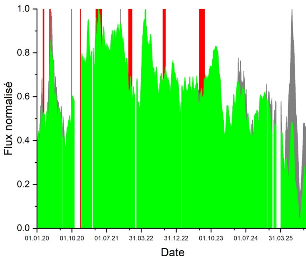
Figure 6: Comparison between the normalized average of corrected for short (OVPF-model; 15 days moving average; in green) and long-term influence of environmental parameters (INGV MALFIT model; in dark gray) soil CO 2 flux from all distal stations. Red bars: eruptions; Gray bars: intrusions.
