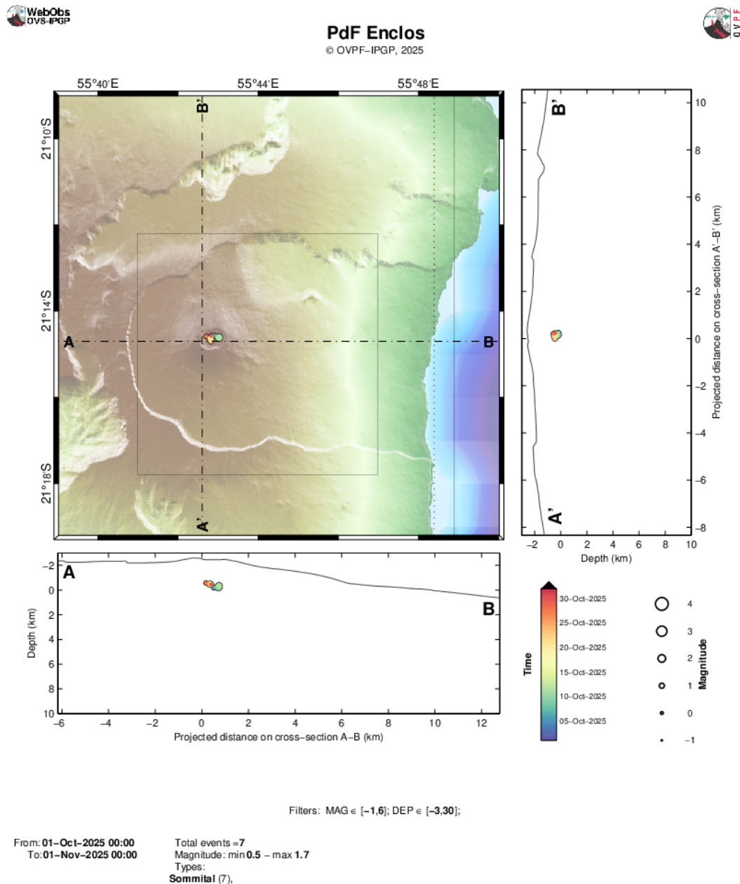
Figure 2: Seismicity below Piton de la Fournaise in October 2025. Location map (epicenters) and north-south and east-west cross-sections (hypocenters) of earthquakes as recorded by OVPF-IPGP. Only manually located earthquakes are shown on the map (© OVPF-IPGP).
