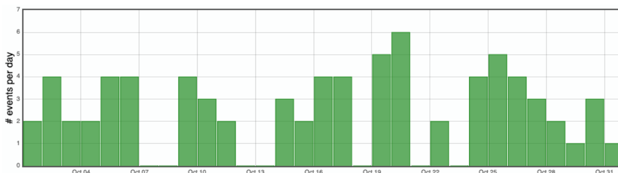
Figure 9: Number of local earthquakes (La Réunion island) per day recorded in October 2025 (© OVPF-IPGP).
