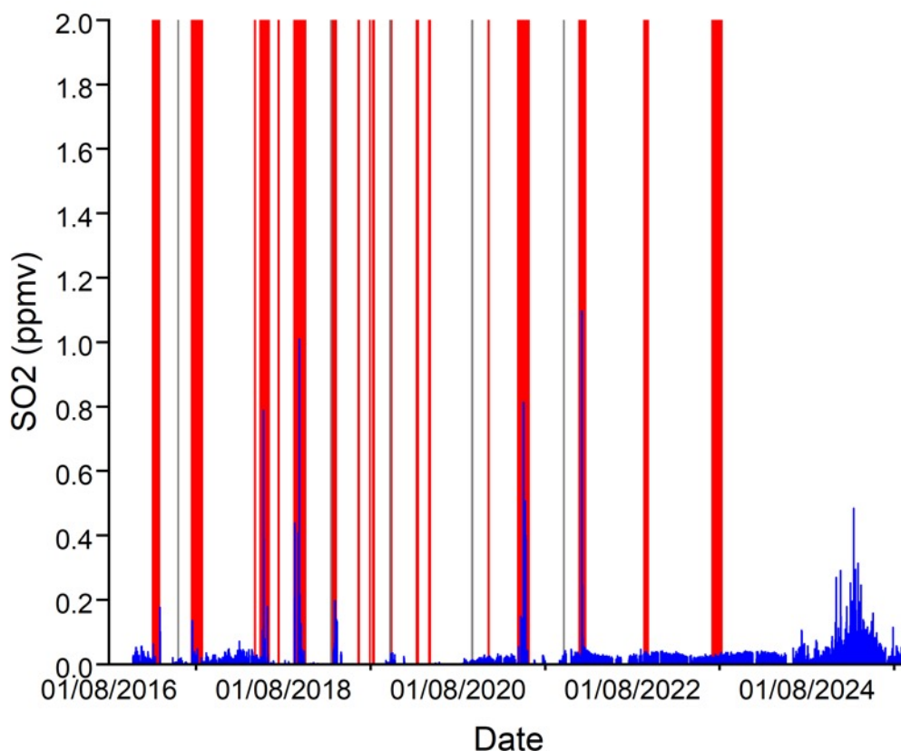
Figure 8: Raw (in blue) concentrations of SO 2 in the atmosphere at the summit of Piton de la Fournaise (MultiGaS station) Red bars: eruptions; Gray bars: intrusions.
