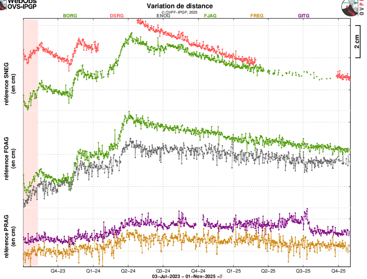
Figure 4: Ground deformation records since the last eruption in July-August 2023 (the eruptive period of July-August 2023 is shown in red). The time series plots show the changes in distance between pairs of GPS stations located around the Dolomieu summit crater (reference: SNEG; top graph), the terminal cone (reference: FOAG; middle graph) and the Enclos Fouqué caldera (reference: PRAG; bottom graph), from north to south (see location in Figure 5). Increasing distances (or baseline elongation) indicate volcano inflation, while decreasing distances (or baseline contraction) reflect edifice deflation (© OVPF-IPGP).
