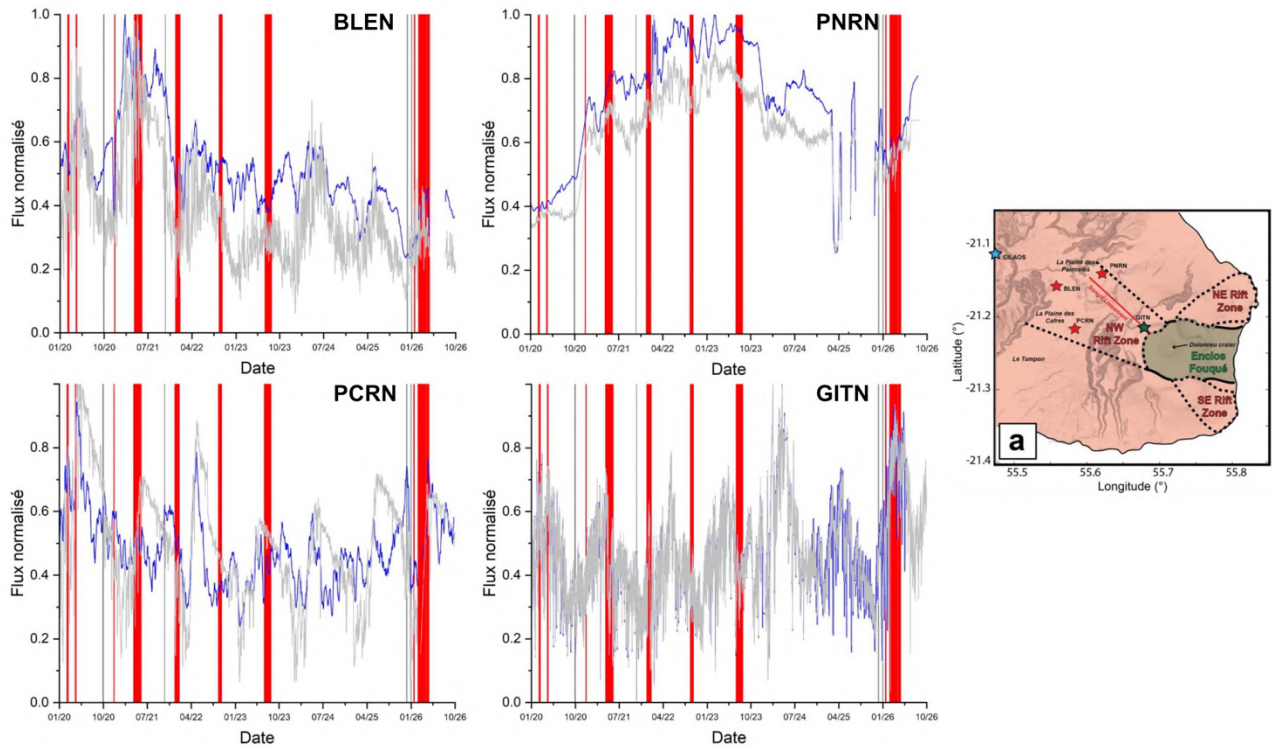
Figure 6: Normalized CO 2 soil emissions (grey: raw data) corrected for short period influence of environmental parameters (OVPF-correction model; 15 days moving average; in blue) of all CO 2 stations (see location on the map on the right). Red bars: eruptions; Gray bars: intrusions (©OVPF-IPGP-OSUL).
