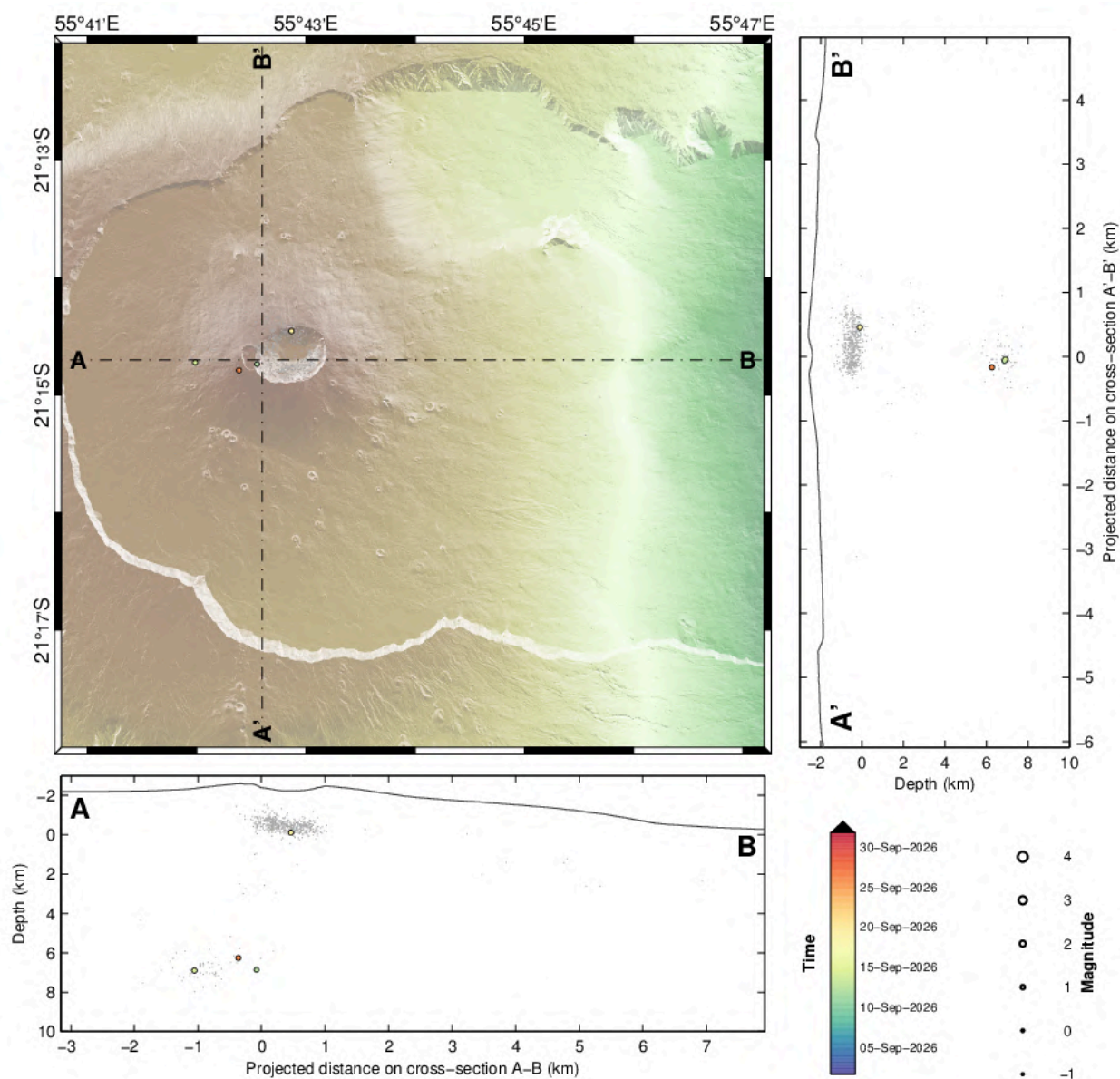
Figure 2: Seismicity below Piton de la Fournaise in September 2026. Location map (epicenters) and north-south and east-west cross-sections (hypocenters) of earthquakes as recorded by OVPF-IPGP. Only manually located earthquakes are shown on the map (©WebObs/OVPF-IPGP).
