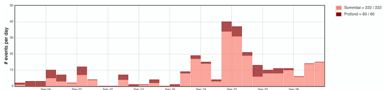
Figure 1: Daily rate of shallow (orange histogram) and deep (red histogram) volcano-tectonic earthquakes per day from the “main courante” catalog in September 2026 (©WebObs/OVPF-IPGP).
