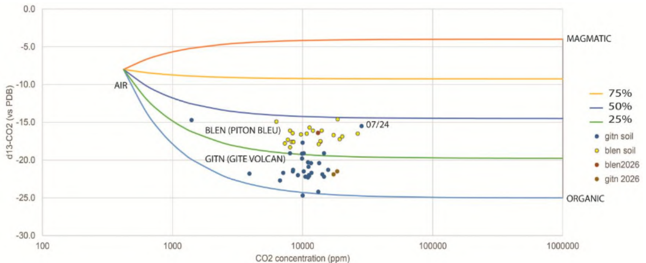
Figure 7: Carbon isotope ( \delta^{13}\text{C} ) variations in CO 2 from soil gas emitted from a proximal (GITN) and distal (BLEN) station. Measurements performed during the main peak (June 2024) at BLEN and at the beginning of the inversion in CO 2 trend at PCRN have recorded the highest percentage of the magmatic contribution.
