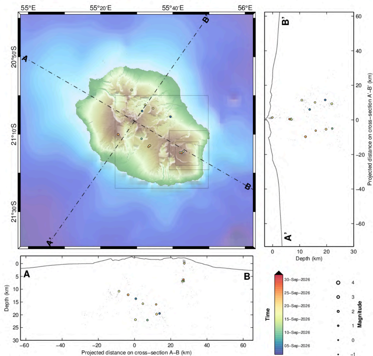
Figure 10: Seismicity below La Réunion in September 2026. Location map (epicenters) and north-west – south-east and south-west – north-east cross-sections (hypocenters) of earthquakes as recorded by OVPF-IPGP. Only localizable earthquakes are shown on the map (©WebObs/OVPF-IPGP).
