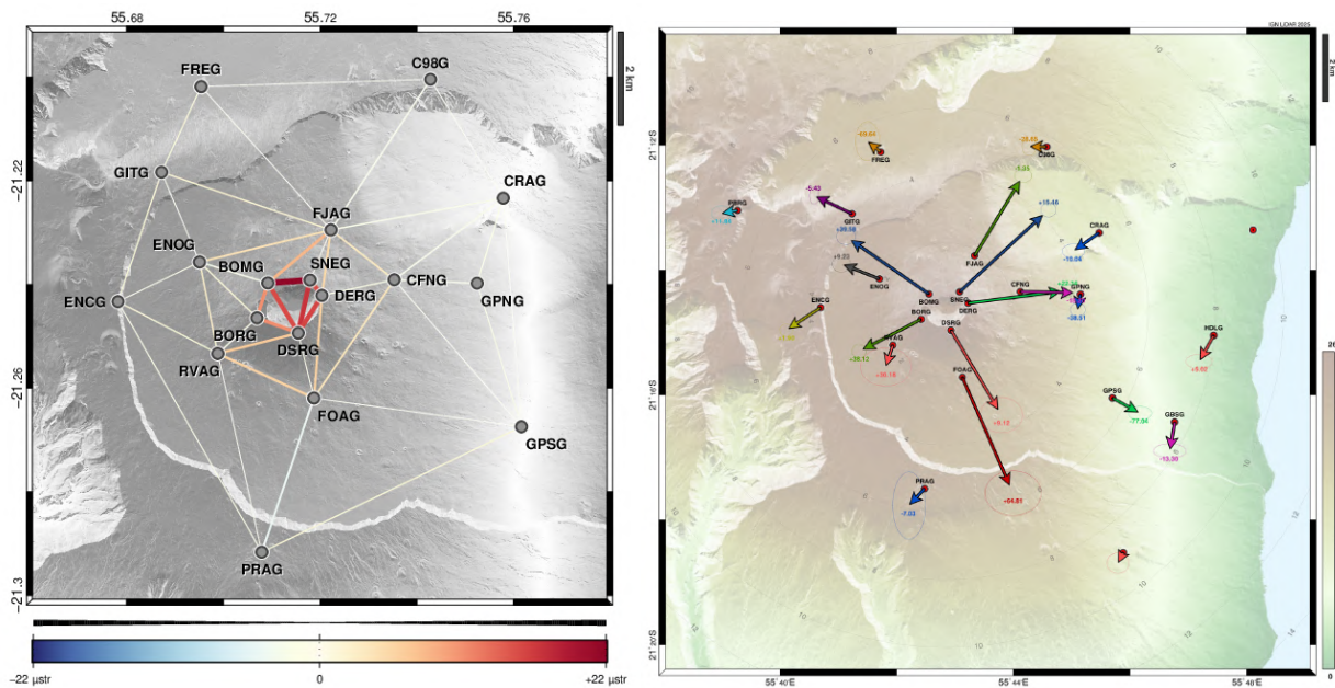
Figure 4: Inflation period of August 1 to September 30, 2026
