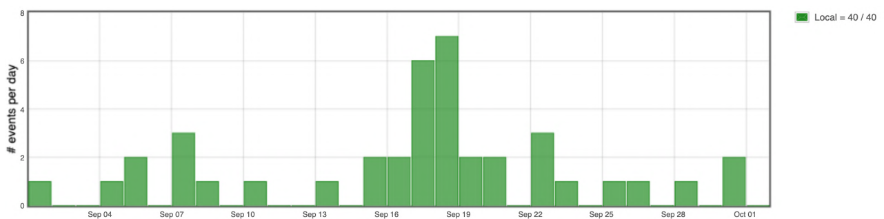
Figure 9: Number of local earthquakes (within a 200 km radius of La Réunion island) per day recorded in September 2026 (©WebObs/OVPF-IPGP).
