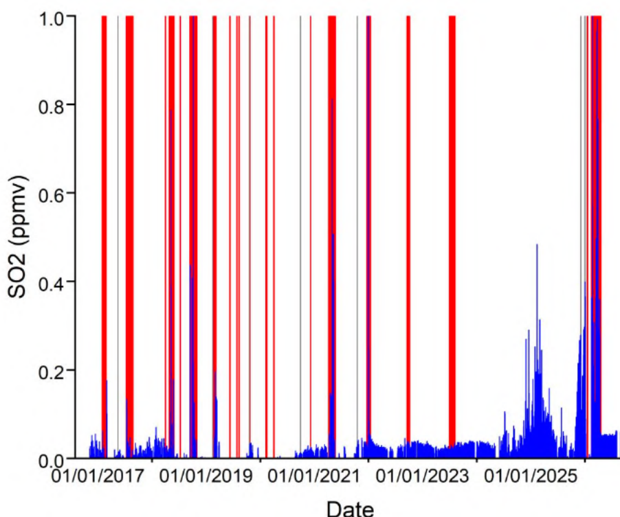
Figure 8: Raw (in blue) concentrations of \text{SO}_2 in the atmosphere at the summit of Piton de la Fournaise (MultiGaS station) Red bars: eruptions; Gray bars: intrusions (©OVPF-IPGP-OSUL).
