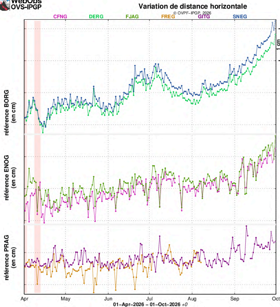
Figure 3: Ground deformation records over the past six months (the red and green bars represent eruptive and intrusive periods, respectively). The time series plots show the changes in horizontal distance between pairs of GNSS stations located around the Dolomieu summit crater (top graph), the terminal cone (middle graph) and the Enclos Fouqué caldera (bottom graph), from north to south (see location on the right). Increasing distances (or baseline elongation) indicate volcano inflation, while decreasing distances (or baseline contraction) reflect edifice deflation (©Webobs/OVPF-IPGP).
