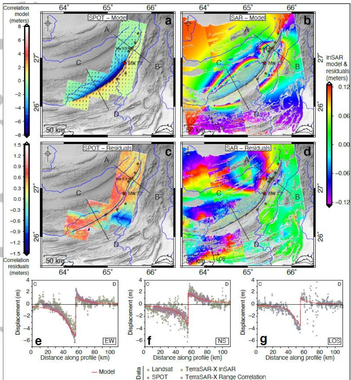
Figure 9. Results from the non-linear inversion. (a-b): Synthetics showing the predicted coseismic horizontal component (a - positive for north-eastward motion) and the projection of coseismic displacements in the TerraSAR-X LOS (b - each color cycle represents 24 cm of LOS displacement). (c-d): residuals. (e-g): profile C-D showing the model predictions (solid lines) along with the data (dots) for 3 components (EW (e), NS (f), TerraSAR-X LOS (g)). Fault trace from Vallage et al. (2016), epicenter from Barnhart et al. (2014), aftershock epicenters from USGS, focal mechanisms from USGS, Geoscope and Global CMT.
