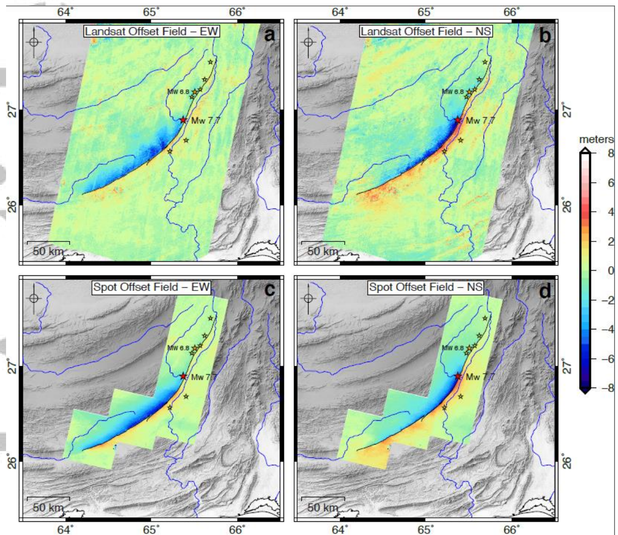
Figure 2. East-west and north-south displacement field (m) for the Balochistan earthquake measured from correlation of pre-earthquake and post-earthquake Landsat (a & b) and SPOT (c & d) optical images. Displacements are positive eastward (a & c) and northward (b & d). Data from Vallage et al. (2015), fault trace from Vallage et al. (2016), main shock epicenter from Barnhart et al. (2014), aftershock epicenters from USGS.
