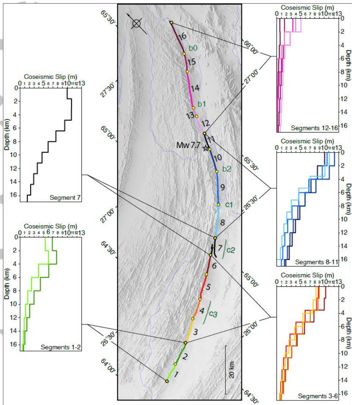
Figure 15. Mean slip as a function of depth for the 16 segments of the Hoshab fault. Complexities from Vallage et al. (2015), fault trace from Vallage et al. (2016), epicenter from Barnhart et al. (2014).
