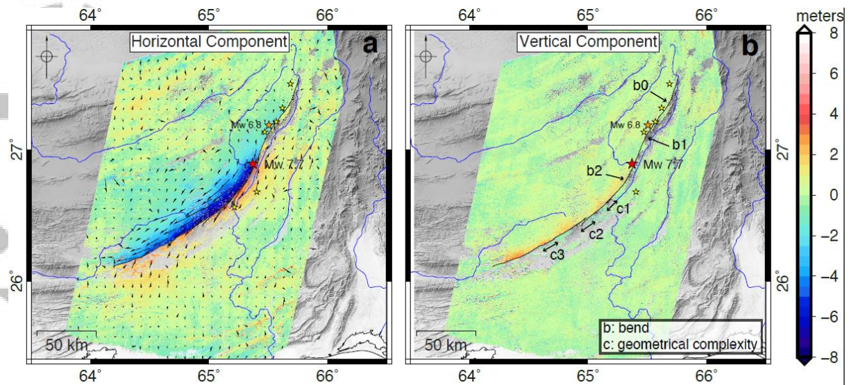
Figure 4. 3D solution for surface deformation obtained from joint analysis of InSAR, radar correlation and optical correlation: horizontal (a - positive for north-eastward motion) and vertical (b - positive for upward motion) displacement fields. Fault trace from Vallage et al. (2016), complexities and bends from Vallage et al. (2015), epicenter from Barnhart et al. (2014), aftershock epicenters from USGS.
