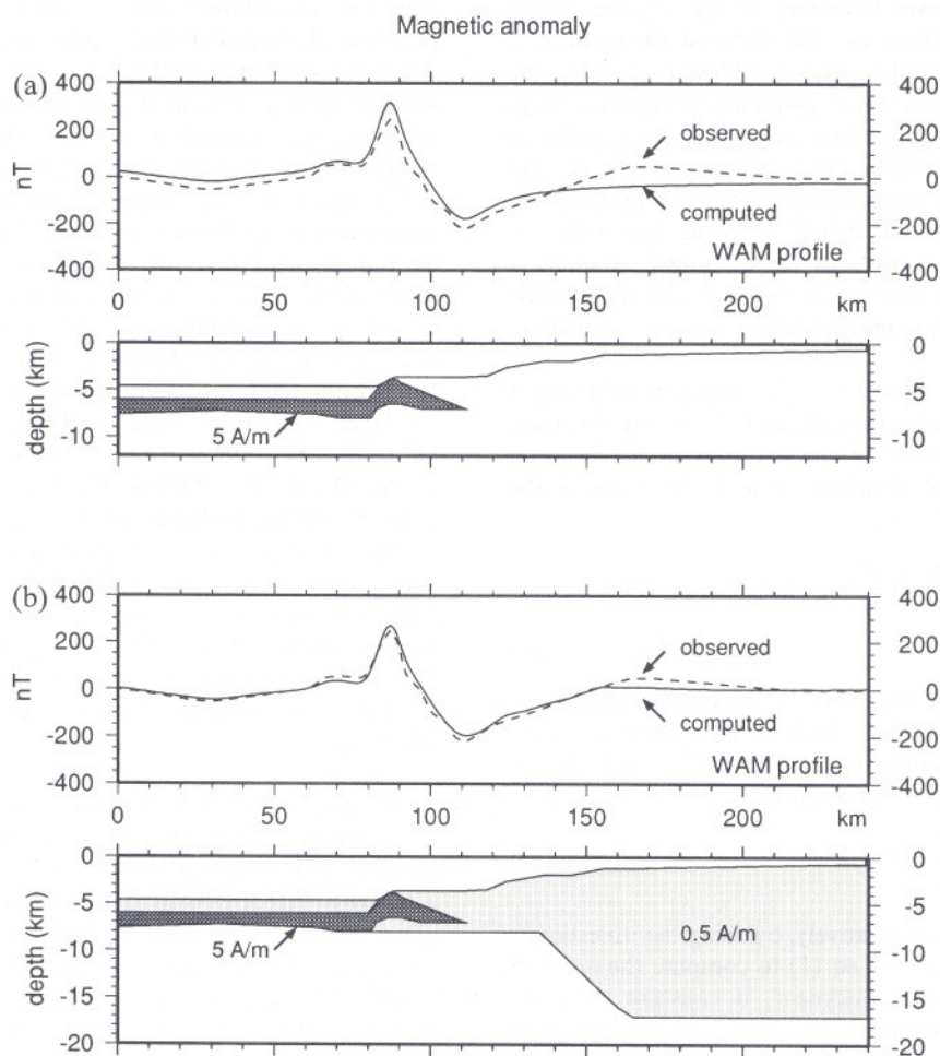
Figure 3. Forward modelling of magnetic anomalies along profile WAM, observed (dashed line) and computed (solid line). (a) a single magnetic body which represents the oceanic domain and the basaltic unit with a magnetization of 5 \text{ A m}^{-1} , and (b) two magnetic bodies which represent the oceanic crust and basaltic unit with a magnetization of 5 \text{ A m}^{-1} and the continental crust with a magnetization of 0.5 \text{ A m}^{-1} .
