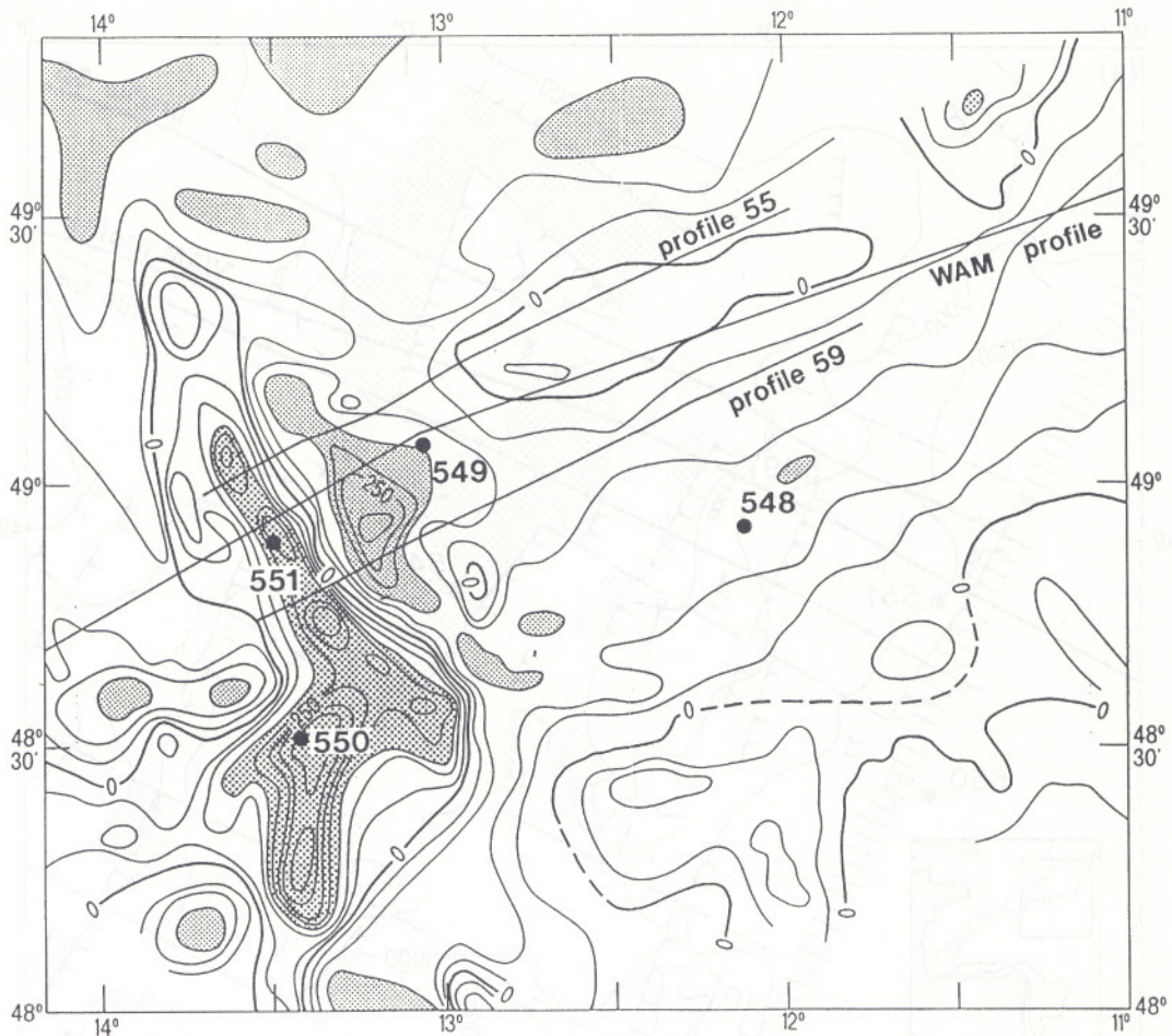
Figure 2. Magnetic-anomaly map of the Goban Spur area (Sibuet 1987) established from marine data. The contour interval is 50 nT. Dotted areas correspond to anomalies higher than 150 nT, fine dotted areas to anomalies lower than 150 nT. The horizontal extension of the volcanic sill located on the deepest tilted block is underlined by an elongated NW–SE anomaly.
