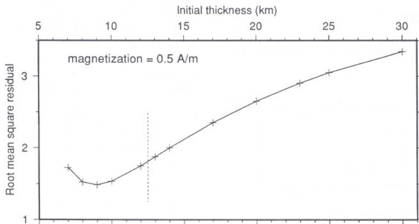
Figure 5. Root-mean-square residual between observed and computed magnetic anomalies versus the initial depth assuming a magnetization of 0.5 \text{ A m}^{-1} . For initial thicknesses smaller than 12 km (vertical dotted line), the inversion process leads to negative thicknesses and its results are therefore discarded.
