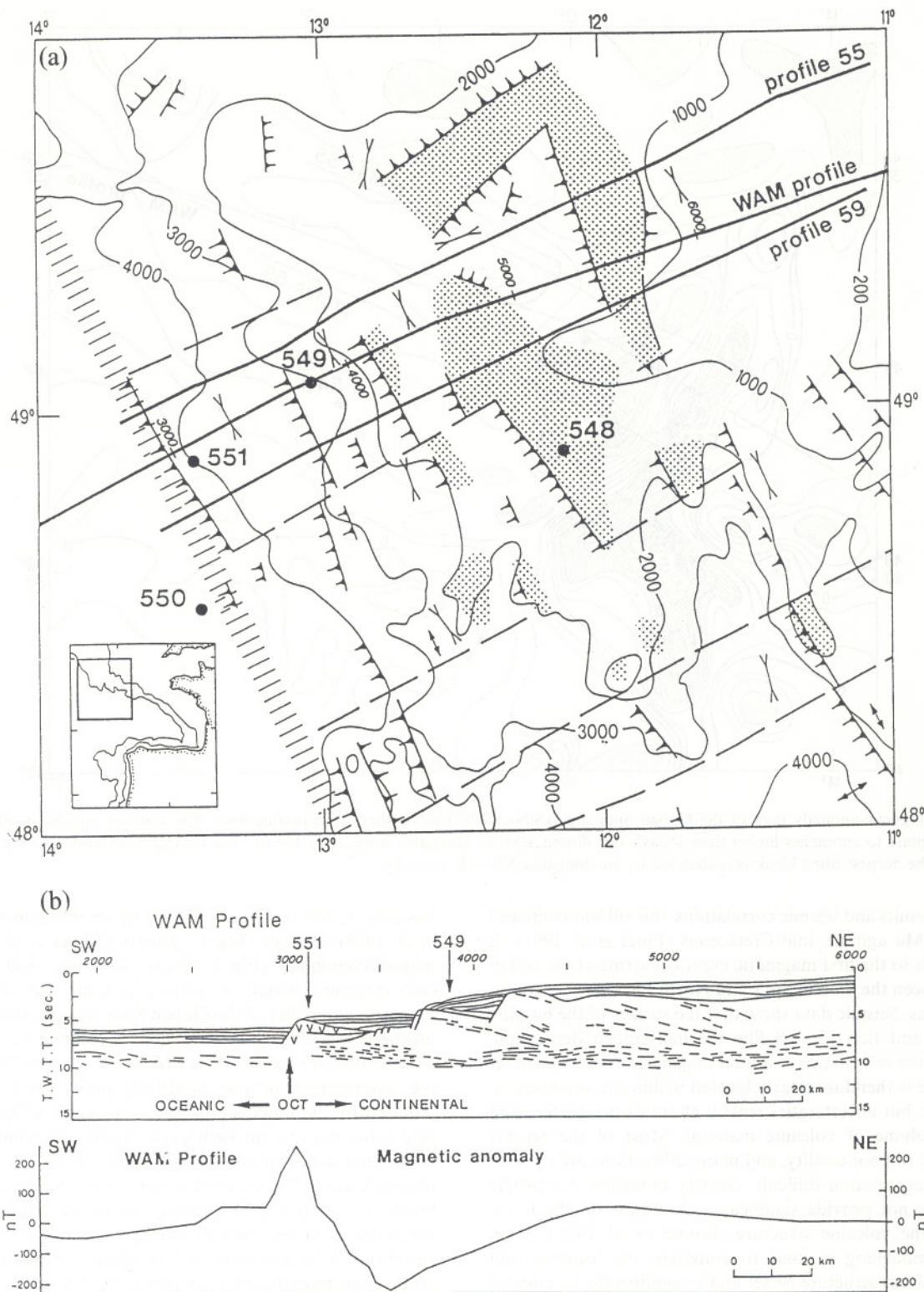
Figure 1. (a) Schematic structural map of the Goban Spur passive margin (Sibuet 1987) with the location of profiles WAM and Norestante 55 and 59. DSDP sites 548–551 are denoted by black dots; long-dashed lines: transverse faults; lines with orthogonal ticks: normal faults; dotted pattern: lower Cretaceous eroded surfaces; dashed pattern: ocean–continent transition. (b) Line drawing of profile WAM and associated magnetic anomaly.
