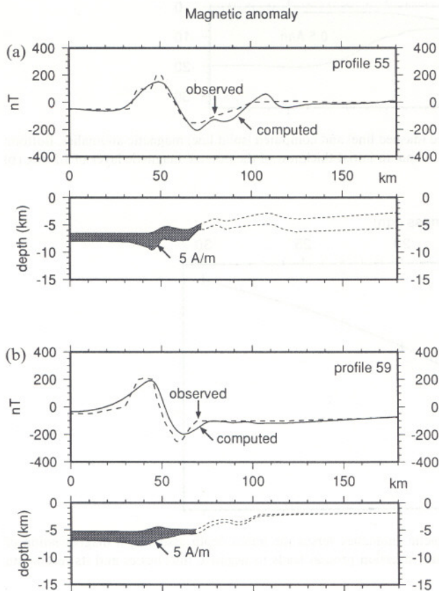
Figure 7. Inversion of magnetic anomalies along profiles Norestlante 55 (a) and 59 (b). Top: observed (dashed line) and computed (solid line) magnetic anomalies. Bottom: magnetic body obtained by inversion assuming a magnetization of 5 \text{ A m}^{-1} and an initial thickness of the oceanic magnetic layer of 2.5 km (a) and 0.5 km (b). Dotted lines show limits of the resulting magnetic body in the continental domain, where a magnetization of 5 \text{ A m}^{-1} is unrealistic.
