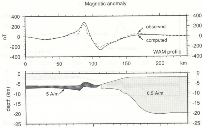
Figure 6. Composite model including results shown on Fig. 4(a) west of km 112 for the oceanic domain and on Fig. 4(b) east of km 112 for the continental domain. The resulting computed magnetic anomaly is in good agreement with the observed one.
