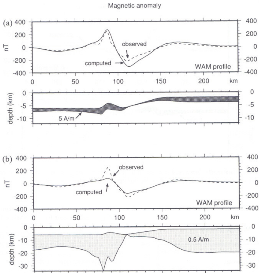
Figure 4. Inversion of magnetic anomalies along profile WAM. Top: observed (dashed line) and computed (solid line) magnetic anomalies. Bottom: magnetic body obtained by inversion assuming (a) a magnetization of 5 \text{ A m}^{-1} and an initial thickness of the oceanic magnetic layer of 1.5 km; (b) a magnetization of 0.5 \text{ A m}^{-1} and an initial thickness of 13 km.
