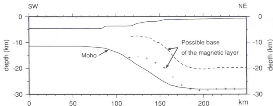
Figure 8. Comparison between the Moho obtained by seismic refraction data and gravity modelling (solid line), and the base of the magnetic layer computed by inversion with maximal thicknesses of 17 km (dashed line) and 28 km (crosses) along profile WAM.
