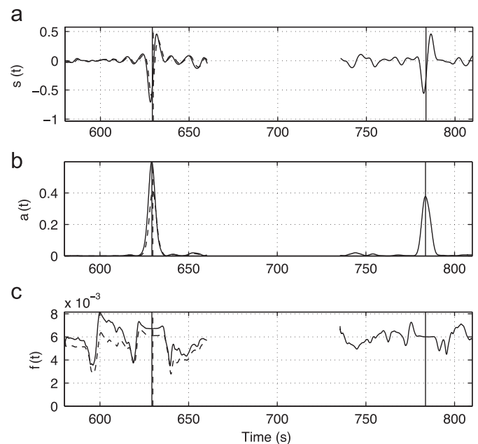
Fig. 1. Instantaneous frequency matching (IFM) method. First, we pick the S and ScS seismic phases by taking the maximum of the envelope (middle panel). Then we compute the instantaneous frequency and compare its value in the time domain at the arrival times of the two seismic waves. The S wave is attenuated using the causal operator D(\omega) , Eq. (2), in the frequency domain for a range of \delta t_{\text{ScS-S}}^* until the instantaneous frequencies are matched in the time domain. The dashed lines correspond to the attenuated seismogram, amplitude and instantaneous frequency. The \delta t_{\text{ScS-S}}^* in this example is 0.6 s. (a) Filtered [0.018 0.2] Hz and anisotropy corrected seismograms, (b) envelope and (c) instantaneous frequency (Hz).
