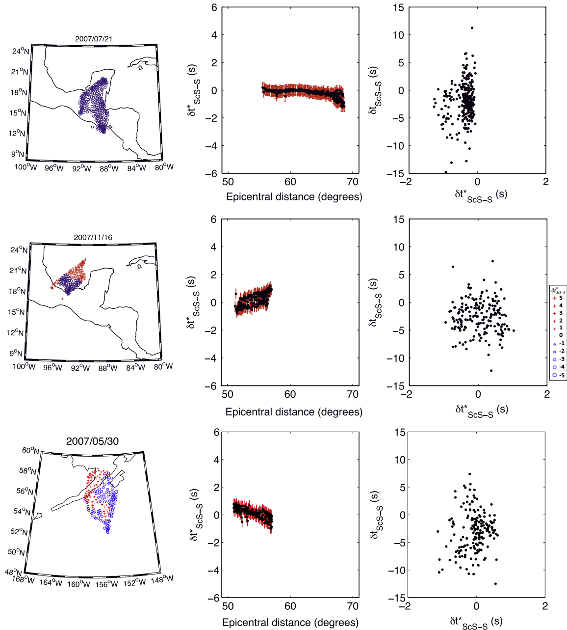
Fig. 6. Stacked anelastic delay times. (left column) Measurements plotted at the reflection point of the ScS on the CMB. (middle column) Measured \delta t_{\text{ScS-S}}^* versus epicentral distance. (right column) Elastic delay-times \delta t_{\text{ScS-S}} versus anelastic delay-times \delta t_{\text{ScS-S}}^* . Both quantities have been corrected using PREM and SAW24B16 for the propagation. The stacking highlights the revealed trends of the \delta t_{\text{ScS-S}}^* with the epicentral distance. No clear correlation is found between elastic and anelastic delay times.
