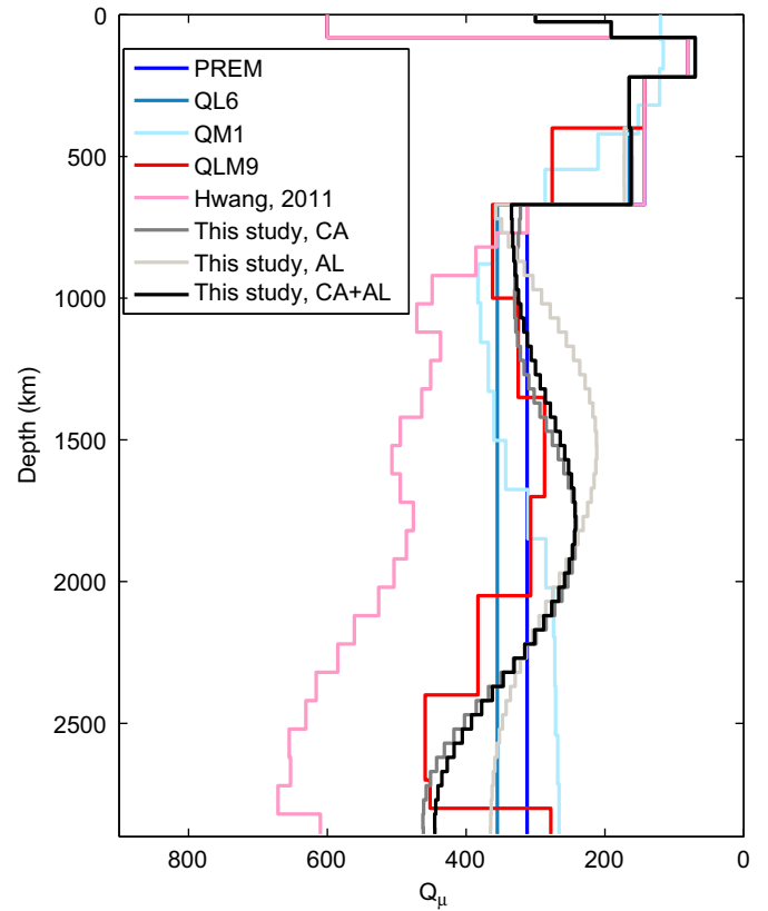
Fig. 8. Various radial Q_\mu models in the mantle. Our models (grey and black lines, CA for Central America and AL for Alaska) bear some similarities with the other body wave based models (red and blue curves) with a less attenuating bottom part of the lower mantle where the normal mode based models are more uniform. (For interpretation of the references to color in this figure caption, the reader is referred to the web version of this article.)
