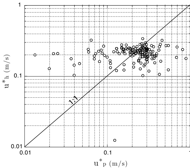
Figure 10 Different estimates of the shear velocity. U_h^* is computed from the average velocity profiles (Eq. (4)), U_p^* is computed by fitting the law of the wall (Eq. (3)).
