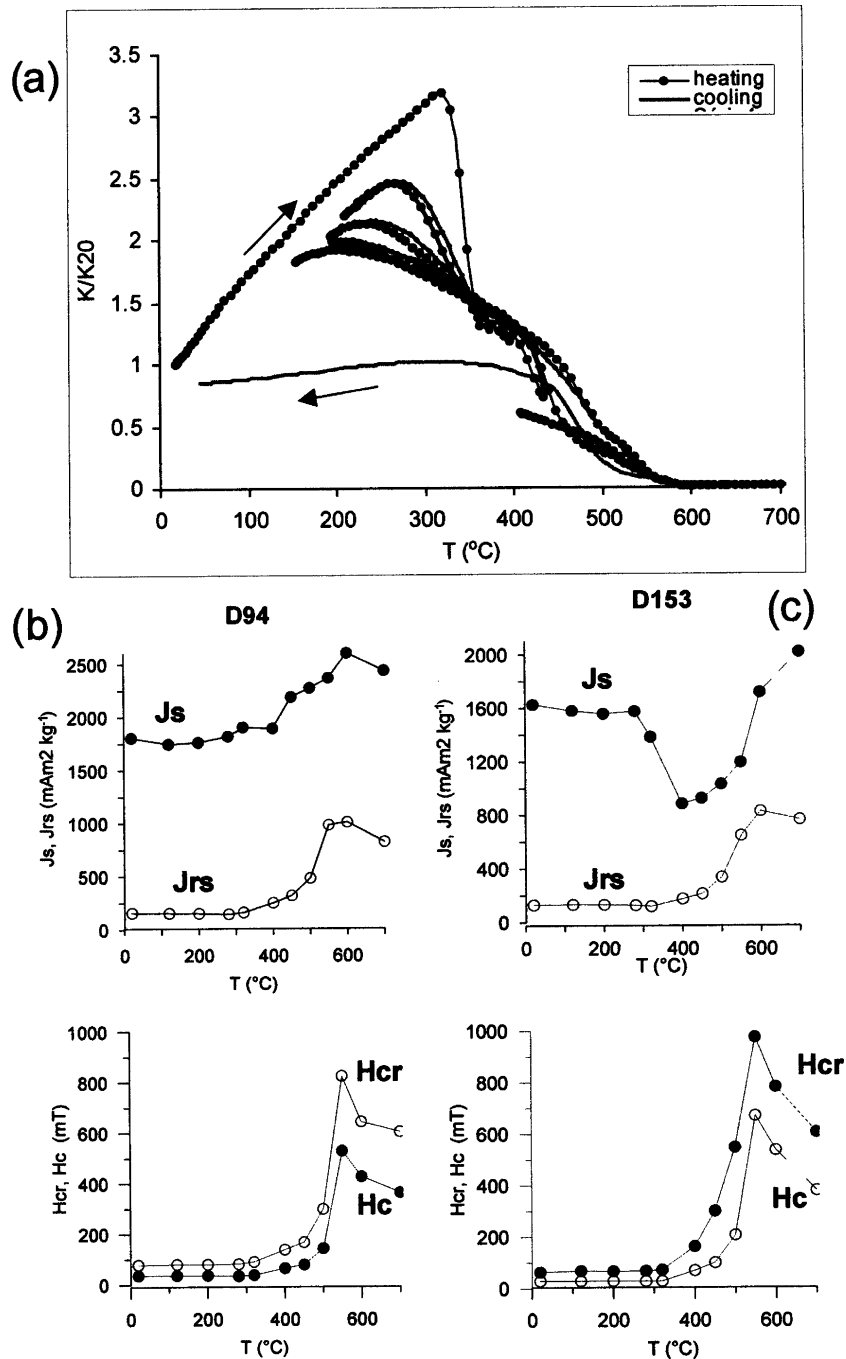
Figure 11. Thermomagnetic K(T) analysis for the dolerite sample D94 (a), and variations of the absolute values of the hysteresis parameters ( J_s , J_{rs} , H_c , H_{cr} ) measured after successive heating steps for samples D94 (b) and D153 (c).
