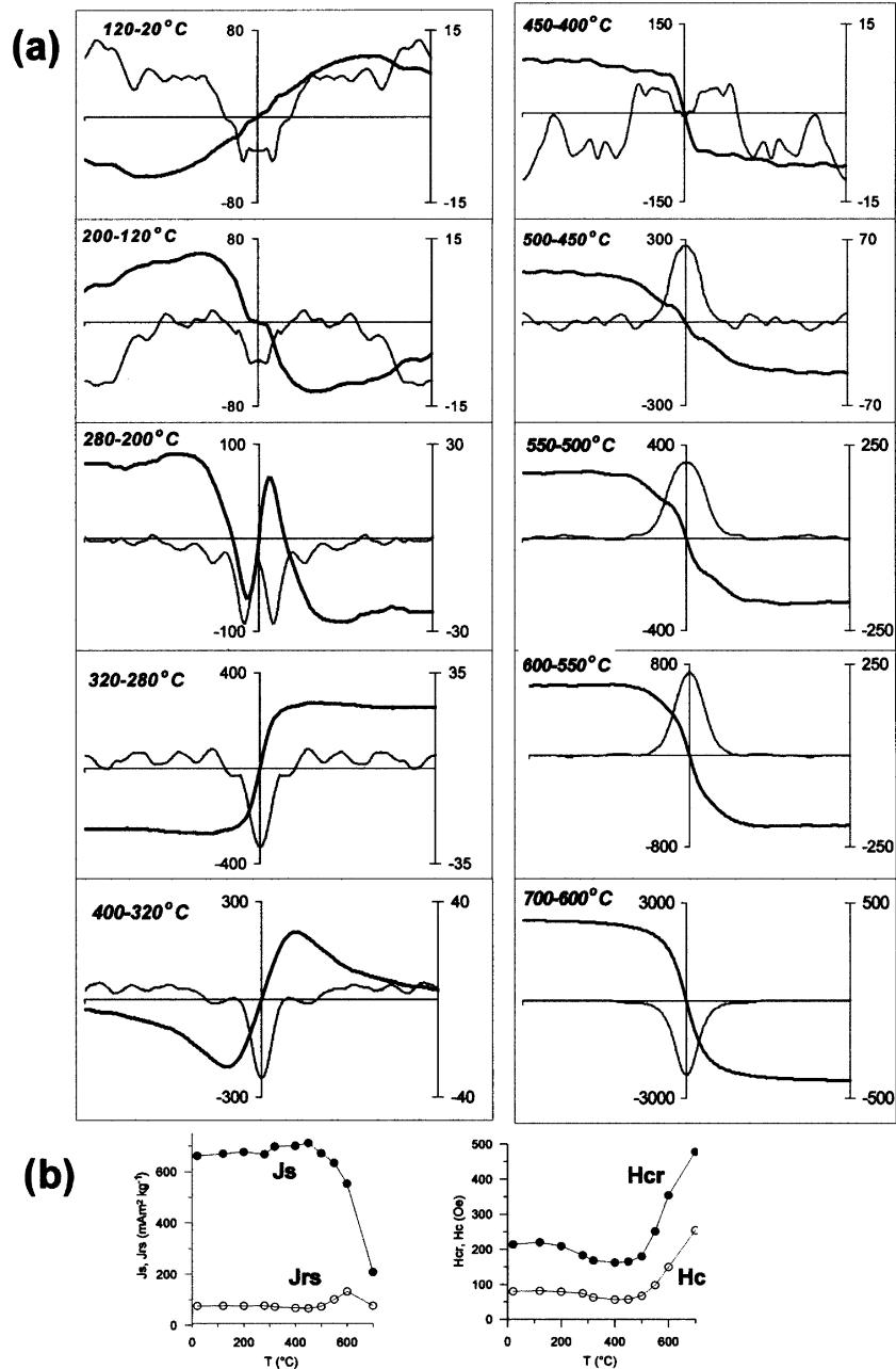
Figure 15. Results obtained for volcanoclastic sandstone (sample D475). (a) Difference loops (induced curve in grey, remanent in black). Field is in T, magnetization in \text{mA m}^2 \text{kg}^{-1} , scale in the middle and on the right for induced and remanent curves respectively. (b) Variations of the absolute values of the hysteresis parameters ( J_s , J_{rs} , H_c , H_{cr} ) measured after successive heating steps.
