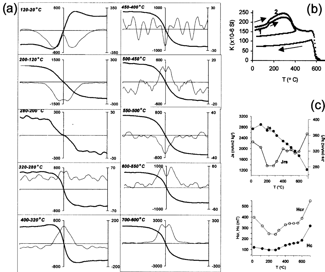
Figure 9. Results for sample KD2A. (a) Difference loops (induced curve in grey, remanent in black; field is from -0.5 to 0.5 T and magnetization in \text{mA m}^2 \text{ kg}^{-1} , scale in the middle and on the right for induced and remanent curves respectively); (b) thermomagnetic K(T) analysis in air for two samples (indicated 1 and 2); and (c) variations of the absolute values of the hysteresis parameters ( J_s , J_{rs} , H_c , H_{cr} ) measured after successive heating steps.
