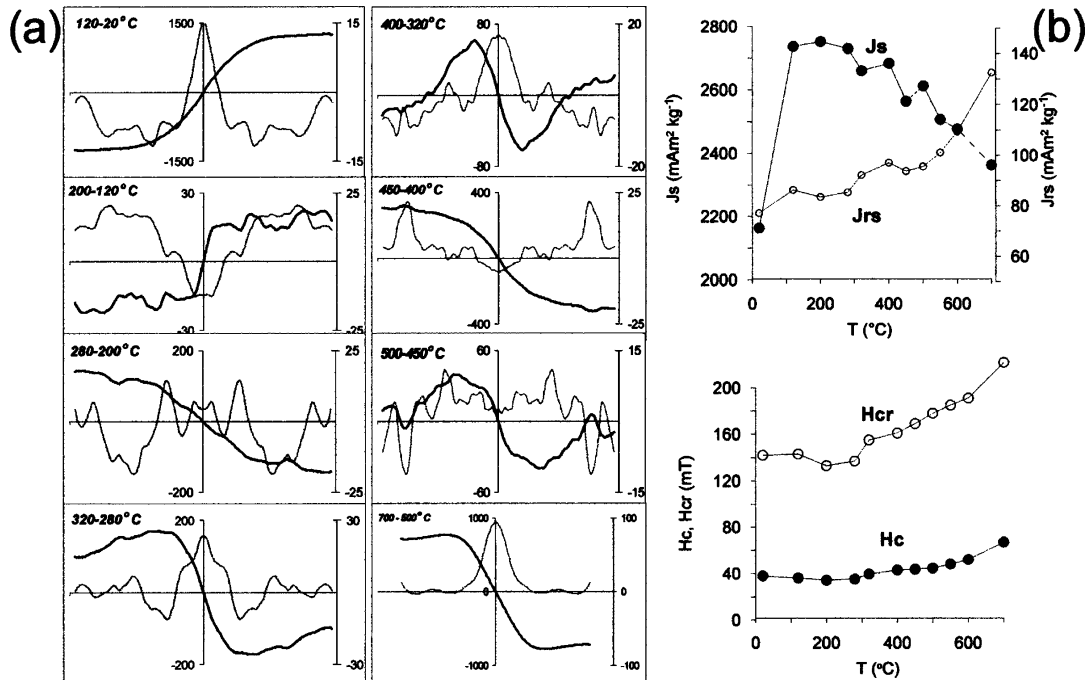
Figure 10. Results for sample H03. (a) Difference loops (induced curve in grey, remanent in black; field is from -0.5 to 0.5 T and magnetization in \text{mA m}^2 \text{ kg}^{-1} , scale in the middle and on the right for induced and remanent curves respectively); (b) variations of the absolute values of the hysteresis parameters ( J_s , J_{rs} , H_c , H_{cr} ) measured after successive heating steps.
