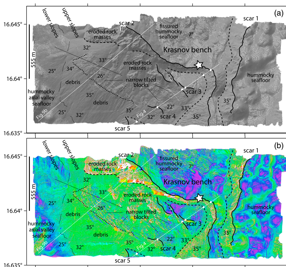
Figure 5. Shaded high-resolution bathymetry (a- with added contours spaced by 2 m in fine grey lines) and slope map (b) for the area of the axial valley wall mapped next to the Krasnov sulphide deposit (star; location in Figure 1b). Color scale for slopes as in Figure 2b. A structural sketch is overlain (see text).
