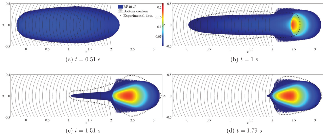
Fig. 31. Test 8: Comparison of the solution of the RP40- \mathcal{J} model with experimental data at several times, the latest one corresponding to the deposit (Coulomb friction law, \delta_0 = 30^\circ ).
