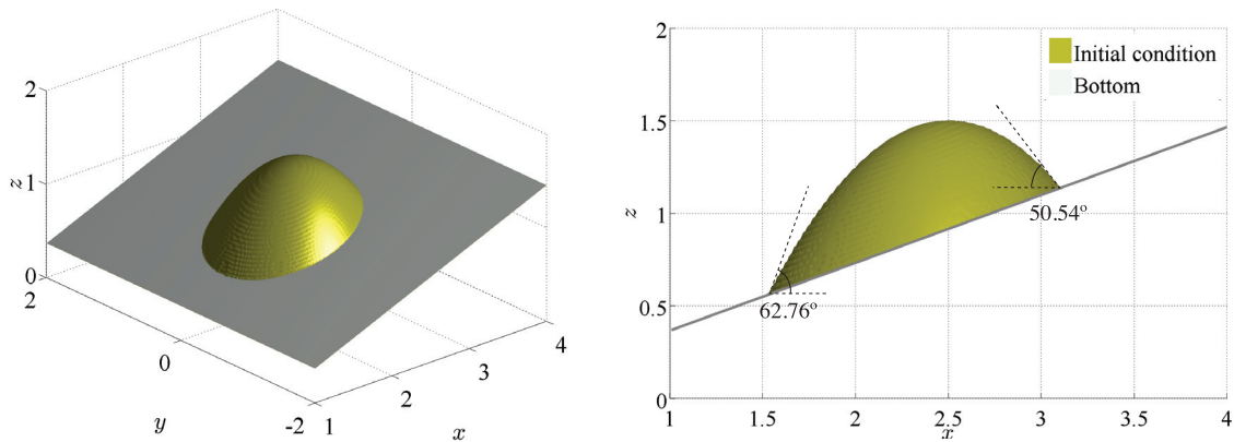
Fig. 25. Test 6. Initial condition and bottom. Left: a 3D perspective. Right: a section of the initial condition when y = 0 .
