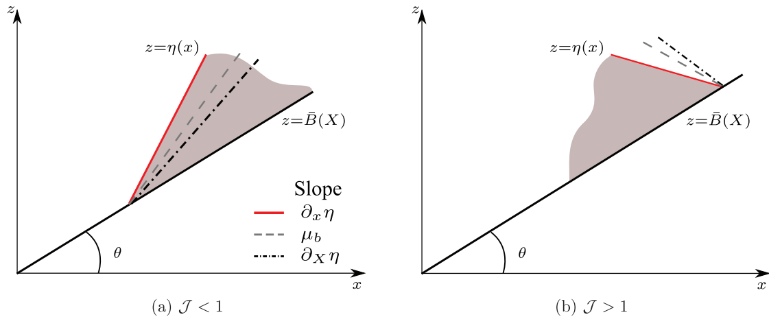
Fig. 3. Pathological situations in the model without correction. Dashed lines have slope \mu_b and dashed-dotted lines have slope \partial_X \eta . Left: a zoom of the front part of the granular avalanche ( \mathcal{J} < 1 ); since |\partial_X \eta| < \mu_b < |\partial_x \eta| , the avalanche should start flowing but the solution of the model will not. Right: a zoom of the rear part ( \mathcal{J} > 1 ); then |\partial_x \eta| < \mu_b < |\partial_X \eta| , so the avalanche should stay at rest but the solution will move upward.
