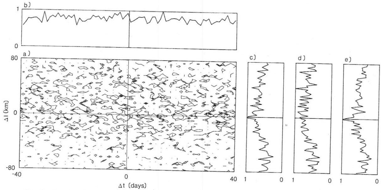
Fig. 12. Second-order moment and correlation functions for the "declustered catalog". (a) Second-order moment m_{21} , corresponding to Figure 3b. Contour interval of 2 is smaller than in Figure 3b due to fewer number of pairs counted in moment for the declustered catalog. (b) Temporal correlation of earthquakes in the "declustered catalog", corresponding to Figure 3c. (c) Spatial correlation of earthquakes in the "declustered catalog" corresponding to Figure 3g. (d) Spatial correlation of earthquakes in the "declustered catalog" for foreshock-main shock parts, corresponding to Figure 3h. (e) Spatial correlation of earthquakes in the "declustered catalog" for main shock-aftershock pairs, corresponding to Figure 3i. See Figure 3 for further explanation.
