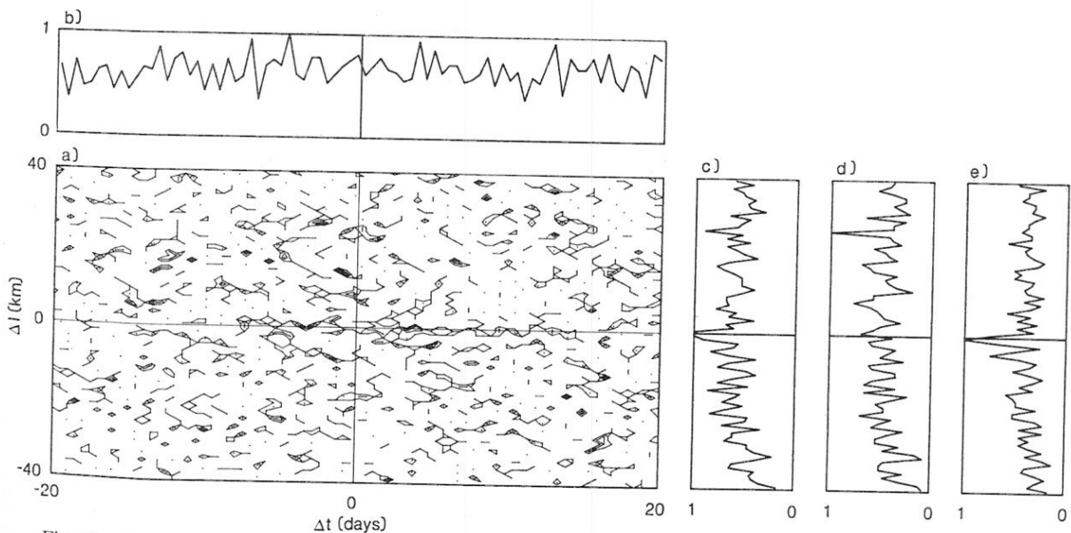
Fig. 13. Second-order moment m_{21} and correlation functions for the "declustered catalog" over the ranges shown in Figure 4.
