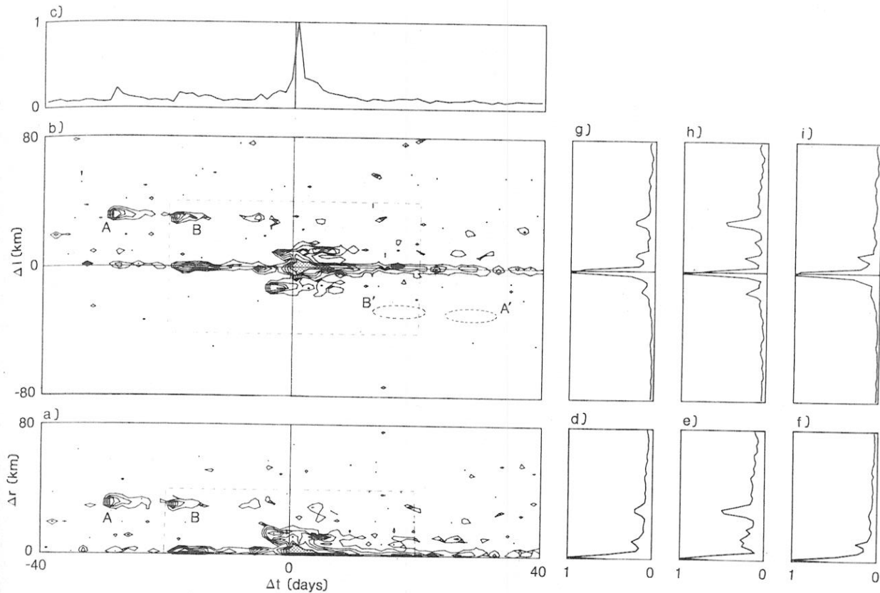
Fig. 3. (a) Second-order moment m_{2r} calculated for the window 0 \leq \Delta r \leq 80 km, -40 \leq \Delta t \leq 40 days, on a 40 (\Delta r) by 80 (\Delta t) grid, shown as contours of number of pairs in the catalog with interevent distance \Delta r and interevent time \Delta t . Each grid point corresponds to a cell 2 km by 1 day. Contour interval is 10. Shading indicates areas with values greater than five contours. Dashed box indicates ranges of moment shown in Figure 4a. Features labeled with a capital letter in Figures 3-5 are discussed in the text. (b) Second-order moment m_{2l} calculated for the window -80 \leq \Delta l \leq 80 km, -40 \leq \Delta t \leq 40 days, on an 80 by 80 grid, shown as contours of number of pairs in the catalog with relative position on the fault \Delta l and interevent time \Delta t (see text). Each grid point corresponds to a cell 2 km by 1 day. Contour interval is 8. Shading indicates areas with values greater than five contours. \Delta l positive (negative) corresponds to pairs in which the smaller event is southeast (northwest) of the main shock. \Delta t positive (negative) corresponds to main shock-aftershock (foreshock-main shock) pairs. Dashed box indicates ranges of moment shown in Figure 4b. (c) Temporal correlation of earthquakes as a function of interevent time \Delta t , obtained by summation of columns in Figure 3b. Time axis corresponds with Figures 3a and 3b. (d) Spatial correlation of earthquakes as a function of interevent distance \Delta r , obtained by summation of rows in Figure 3a. Relative distance axis corresponds with Figure 3a. (e) Same as Figure 3d, but calculated only for foreshock-main shock pairs. (f) Same as Figure 3d, but calculated only for main shock-aftershock pairs. (g) Spatial correlation of earthquakes as a function of relative position along fault \Delta l (see text), obtained by summation of rows in Figure 3b. Relative distance axis corresponds with Figure 3b. (h) Same as Figure 3g, but calculated only for foreshock-main shock pairs. (i) Same as Figure 3g, but calculated only for main shock-aftershock pairs.
