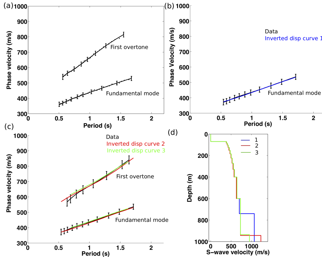
Figure 3. (a) Average phase velocity dispersion curves. Black dots are phase velocity picks measured on the F–K spectra (Figs 2c and d) for the fundamental and first overtone, respectively. Black solid lines with error-bars are the third order polynomial fits of these phase velocities. (b) Comparison between measured (black) and inverted (blue) phase velocities when only the fundamental mode is inverted. (c) Comparison between measured (black) and inverted (green and red) velocities when both fundamental mode and first overtone are inverted. (d) inverted S -wave velocity as a function of depth for the three inversions: when only the fundamental mode is inverted (blue); when the fundamental mode and first overtone are inverted in the period range 0.55 to 1.75 s (red); when the fundamental mode and first overtone are inverted in the period range 0.7 to 1.6 and 1 to 1.5 s, respectively (green).
