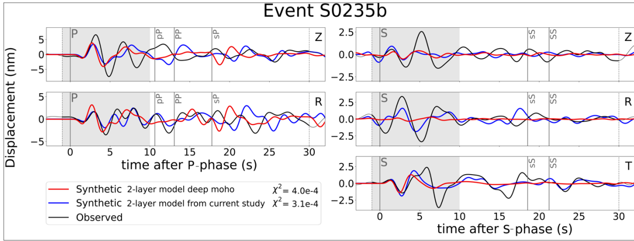
Fig. S20. Source inversion results for event S0235b (black lines show the recorded data) taken from Brinkman et al. (83) for 2 layer-models with the Moho at 80 km (red lines) and 24 km (blue lines). The latter model is equivalent to the 2-layer model of this study. The two left panels represent from top to bottom the vertical (Z) and radial (R) component of the P-waveform. The right three panels show from top to bottom the vertical (Z), radial (R) and transverse (T) component of the S-waveform. The dashed gray lines and area present the total length of the inversion window and higher weighted part of the inversion window, respectively. The solid gray vertical lines denote the first arriving P- and S-waves and later-arriving phases (pP, PP, sP, sS and SS) calculated using ray theory. The misfit value ( \chi^2 ) for each of the inversion is specified in the legend.
