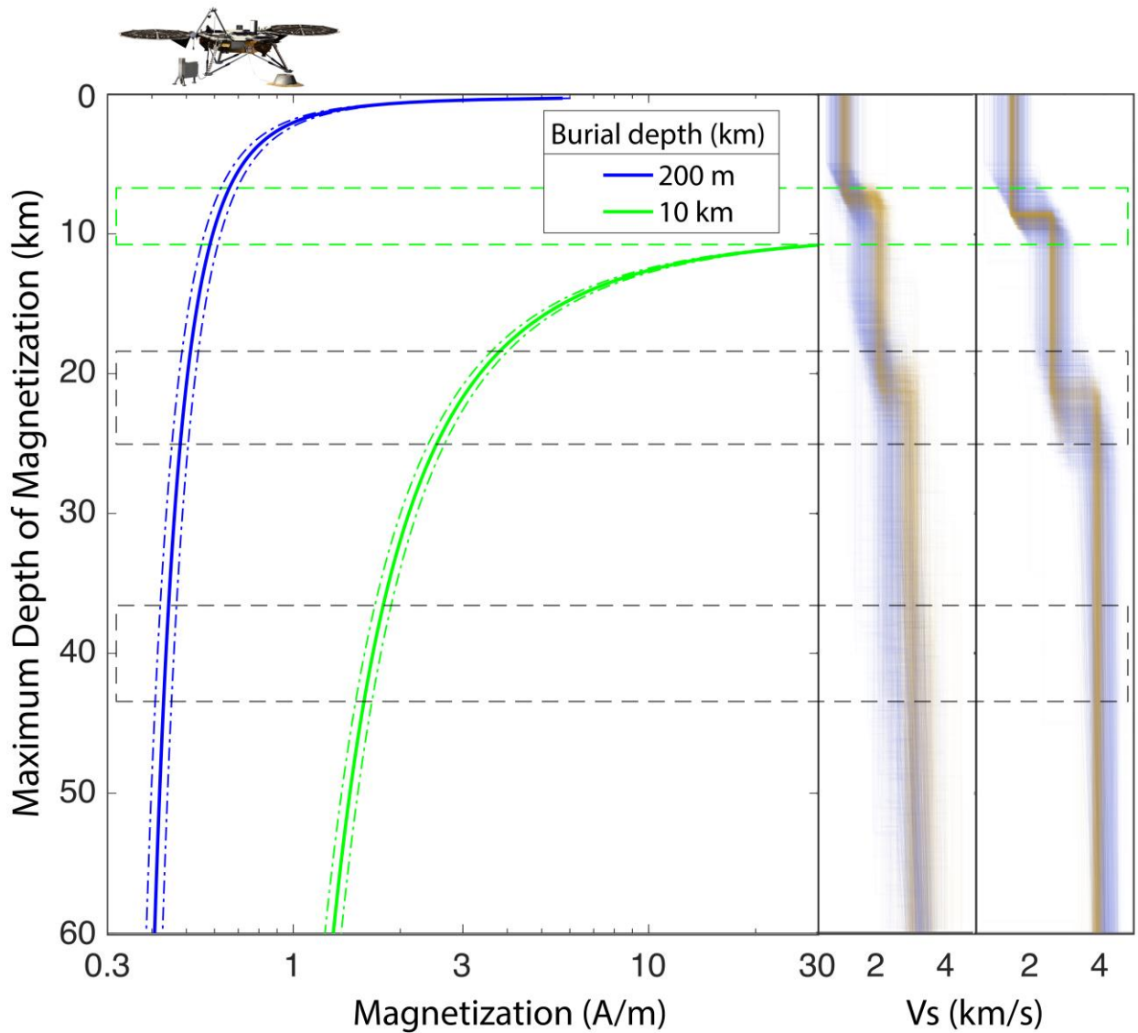
Fig. S28. Estimation of minimum magnetization. The minimum magnetization required from a surface field of 2013 nT and the upper and lower 99% confidence intervals on the surface field strength ( 108 ). Burial depth describes the depth extent of the unmagnetized layers above the top of the magnetized layer. For a burial depth of 200 m (blue), corresponding to burial beneath the young, Amazonian-Hesperian, near-surface lava flows ( 108 ) magnetizations are \sim 0.4 A/m if the entire underlying crust is magnetized. A burial depth of 10 km requires magnetizations larger than 1 A/m. The velocity profiles show the range of seismically-determined interface depths as in Fig. 2 of the main paper.
